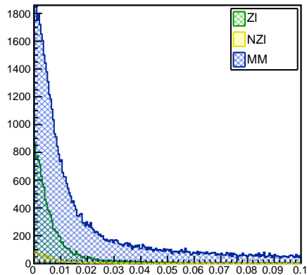
tracks_dzVtx
