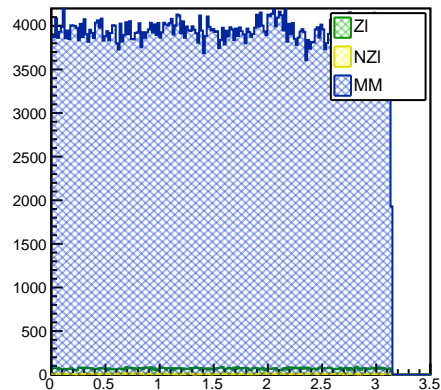
Track Phi
