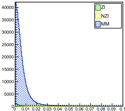
tracks_dxyVtx
