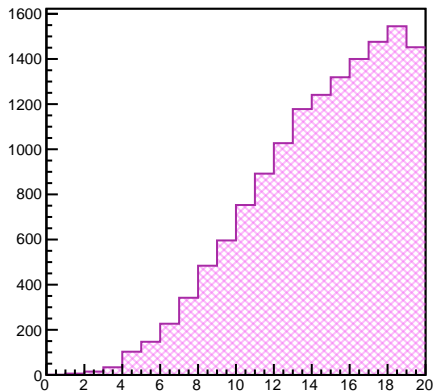
Number of Isolated Tracks
