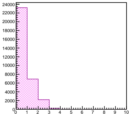
Number of Reco Leptons
