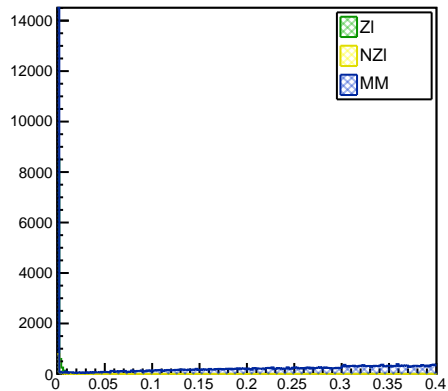
tracks_trackLeptonIso
