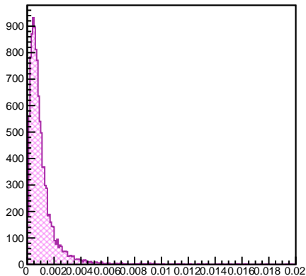
Lepton Min Delta Z
