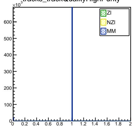
tracks_trackQualityHighPurity
