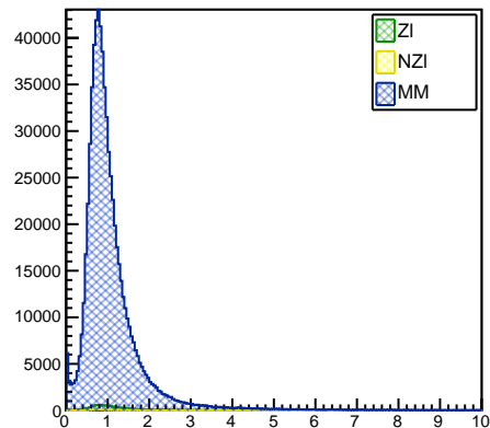
tracks_chi2perNdf
