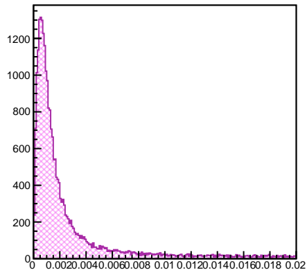
Track Min Delta Z
