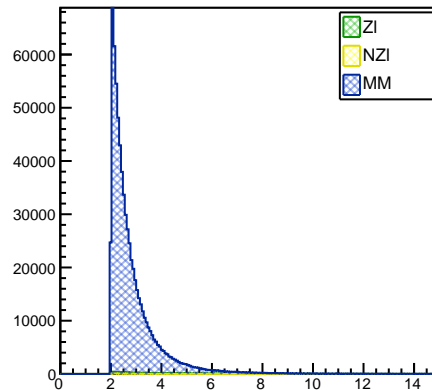
Track Pt
