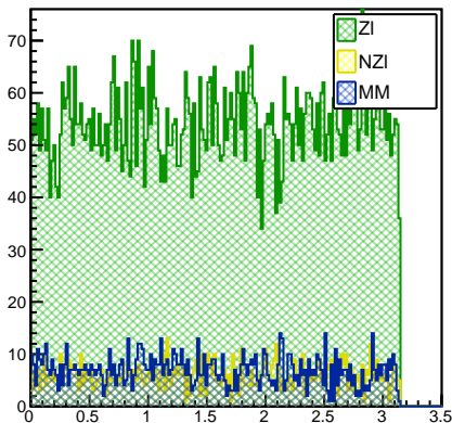
Rec Phi
