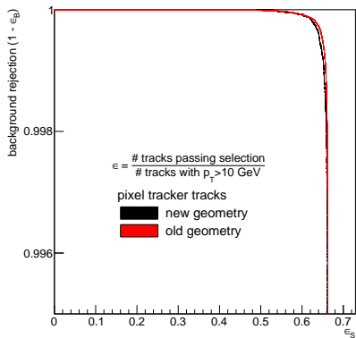
BDT training using old/new geometry MC
