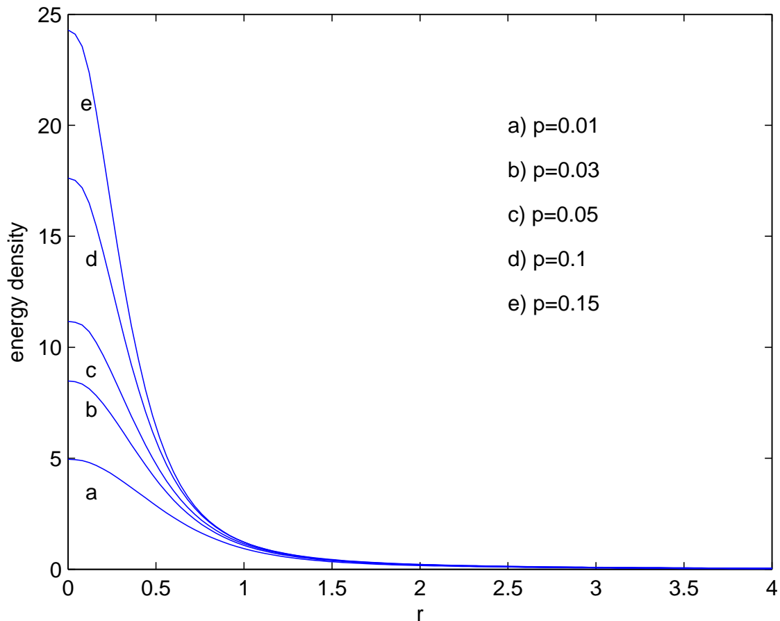
Figure 1: Profiles of energy density \mathcal{H}(r) of the A3M solitons
