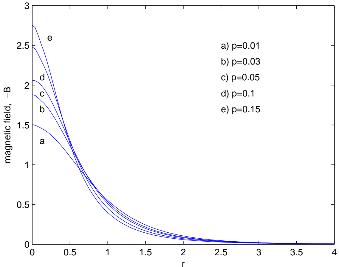
Figure 1: Profiles of magnetic field B(r) of the A3M solitons
