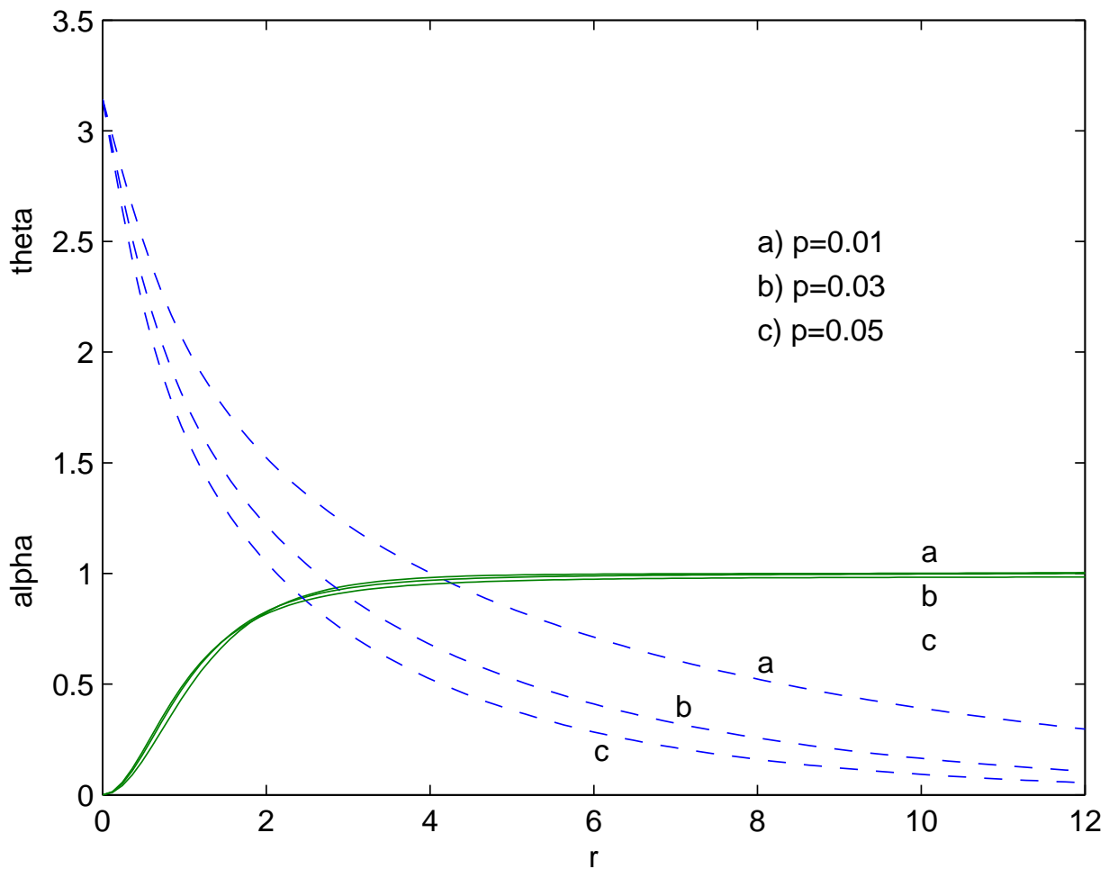
Figure 1: \theta(r) and \alpha(r) of the A3M solitons
