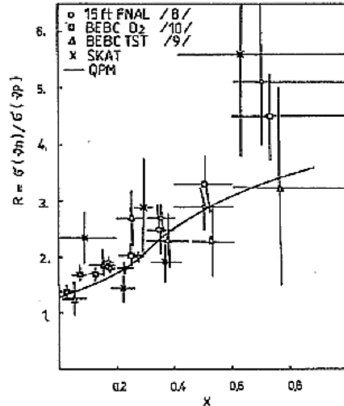
Fig. 4. World data of the dependence of the cross section ratio \sigma(\nu n)/\sigma(\nu p) on Bjorken- x measured in neutrino bubble chamber experiments. The full line gives the prediction of the quark parton model [1, 2] using the parametrisation of the quark distributions by Feynman-Field [5]
