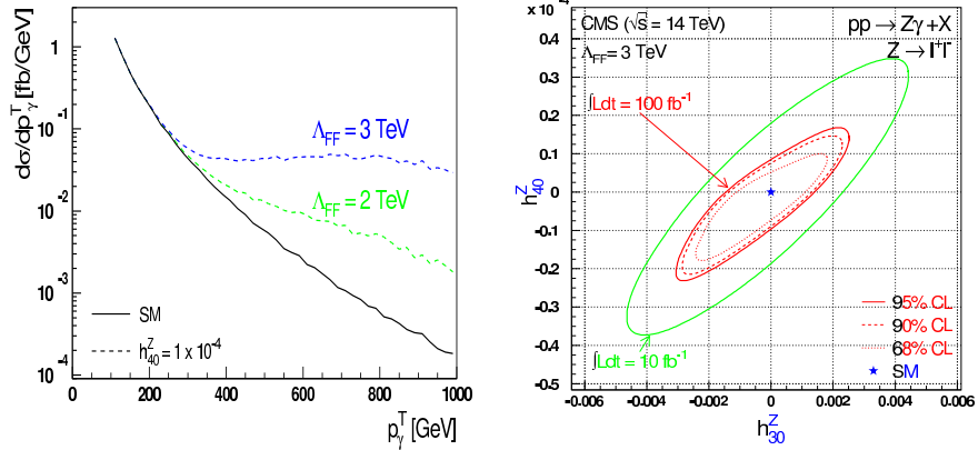
Figure 6: Left: photon p_T of Z\gamma production with h_{40}^Z = 1 \times 10^{-4} and \Lambda = 2 and 3 TeV. Right: the sensitivity contours in the h_{30}^Z , h_{40}^Z parameter space obtained with \Lambda = 3 TeV for 10 and 100 fb -1 of data [13].
