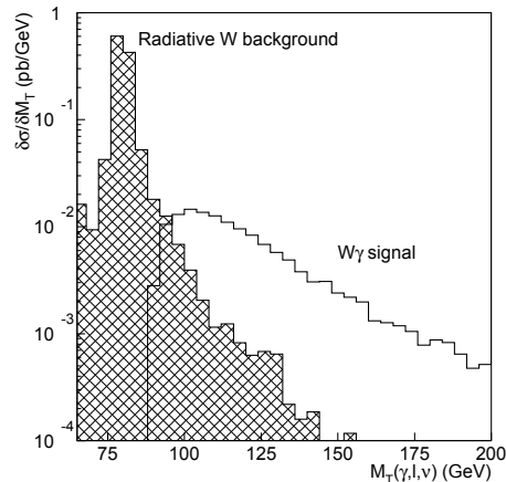
Figure 3: Transverse mass M_T(l, \nu, \gamma) of W\gamma events with a ISR (or WW\gamma ) photon or of radiative W decays with a FSR photon (hatched) [9].
