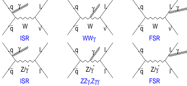
Figure 2: The Standard Model tree-level diagrams for W\gamma and Z\gamma productions at hadron colliders.
