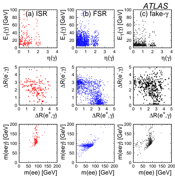
Figure 4: Distributions of Z(ee)\gamma event variables for signal with an ISR photon, and backgrounds with a FSR or a fake photon [6].
