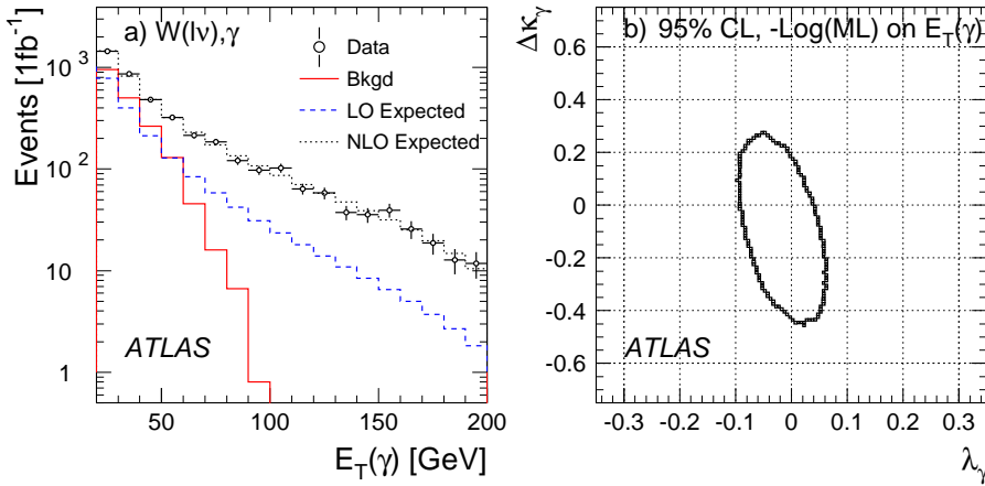
Figure 5: The photon transverse energy distributions of W(l\nu)\gamma ( l = e, \mu ) events, and the 95 % confidence contour extracted in the \Delta\kappa_\gamma , \lambda_\gamma parameter space ( \Lambda = 2 TeV) for 1 \text{fb}^{-1} of data [6].
