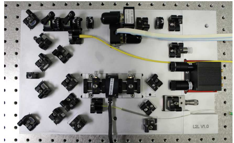
Laser Synchronization (L2L)
