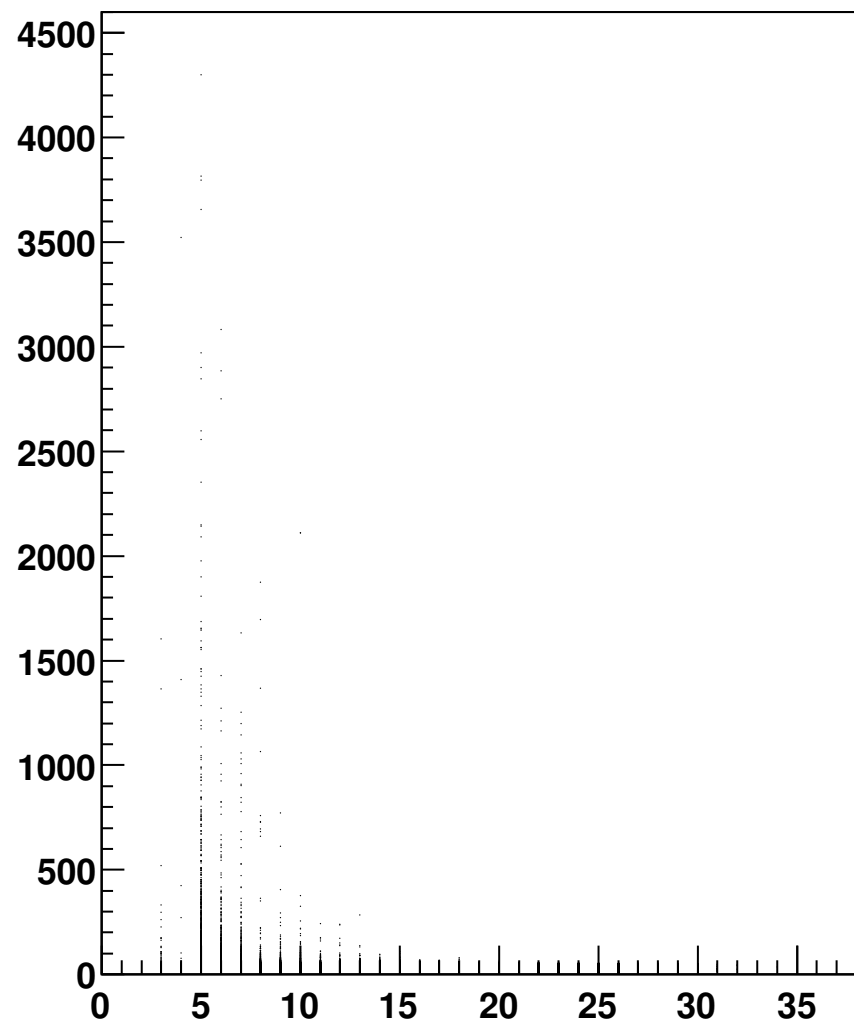
track_p:track_nHits
