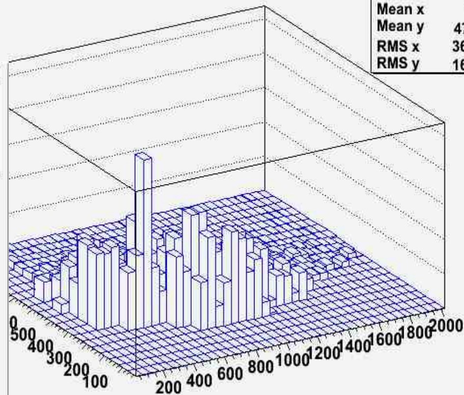
cross_H0-->ttbar
