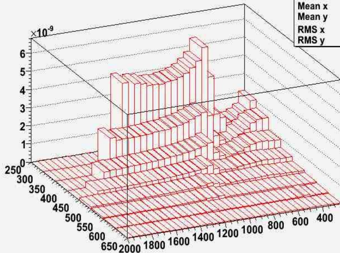
cross_TP_lo
