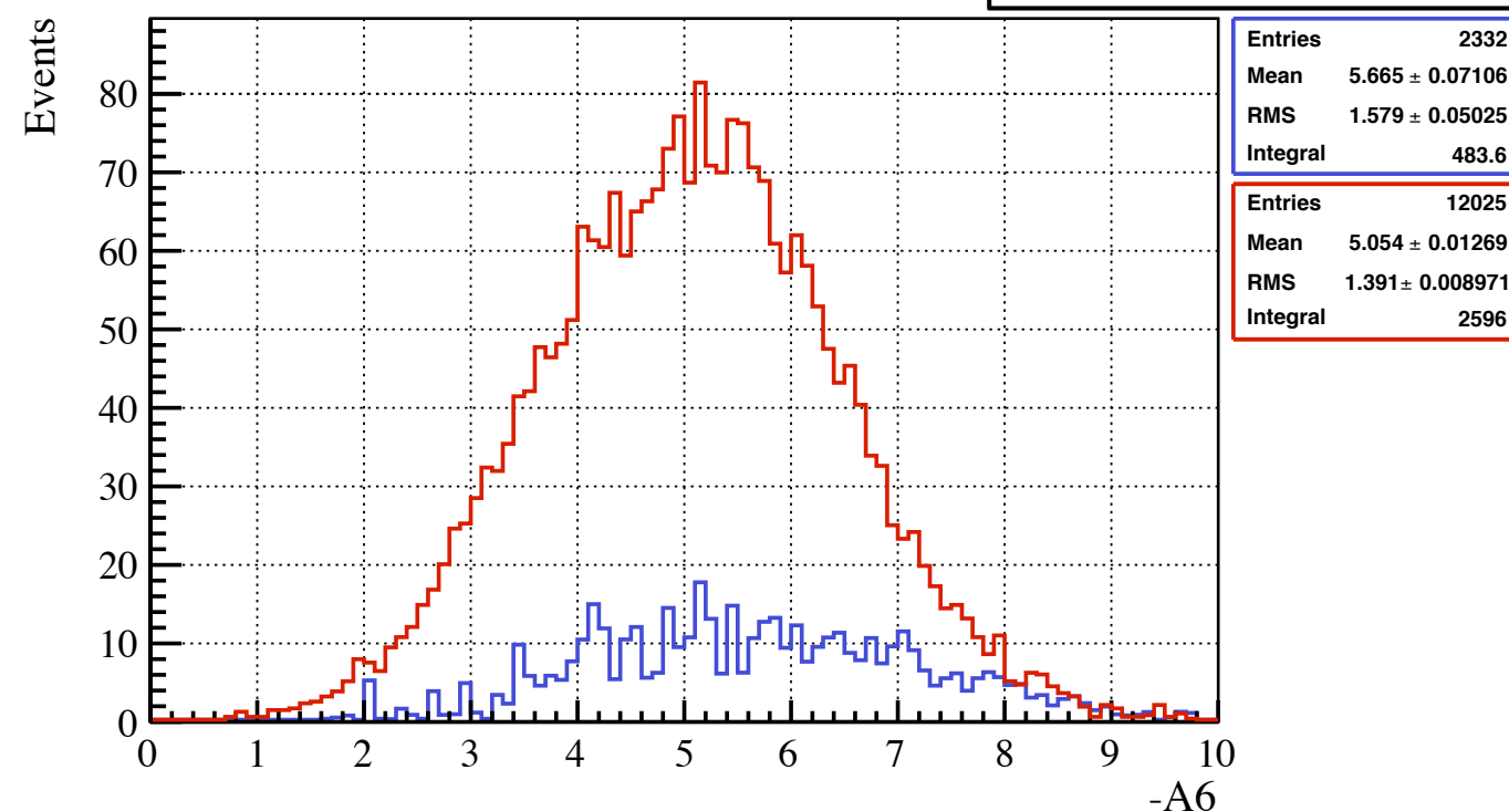
Antenna 6
