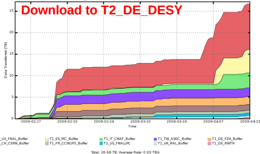
CMS PhEDEx - Cumulative Transfer Volume 90 Days from Week 03 of 2009 to Week 16 of 2009
