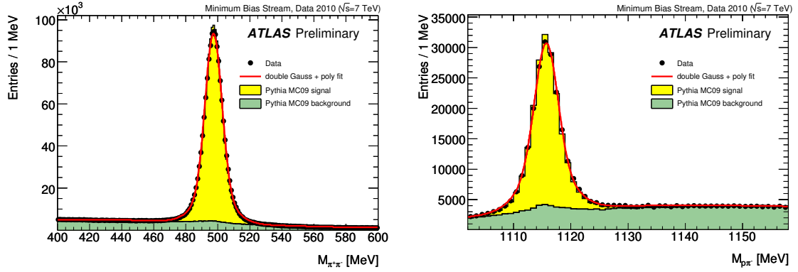
Figure 1: Comparison of measured and predicted K_S^0 (left) and \Lambda (right) mass spectra in the barrel region of the Inner Detector. (Both tracks satisfy |\eta| < 1.2 .) The black circles are data, while the histograms show Monte Carlo simulation (normalised to data). The solid red line is the line-shape function fitted to data.
