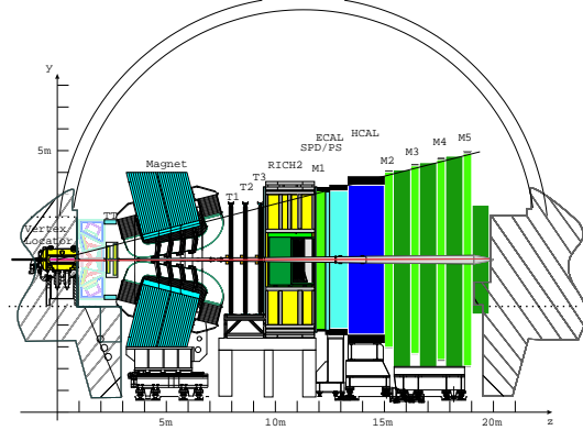
Figure 1: LHCb spectrometer
