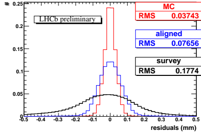
Figure 2: IT residuals
