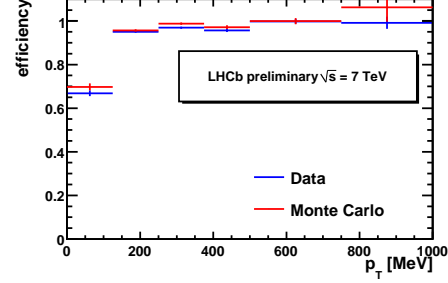
Figure 5: Tracking efficiency vs K_S 's p_T
