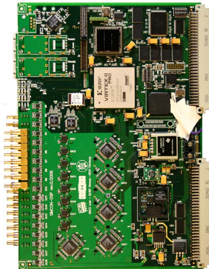
SIMCON DSP Board
