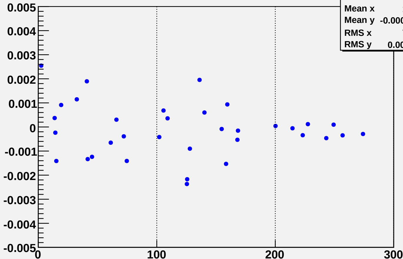
fitted beam splitter angle per beam
