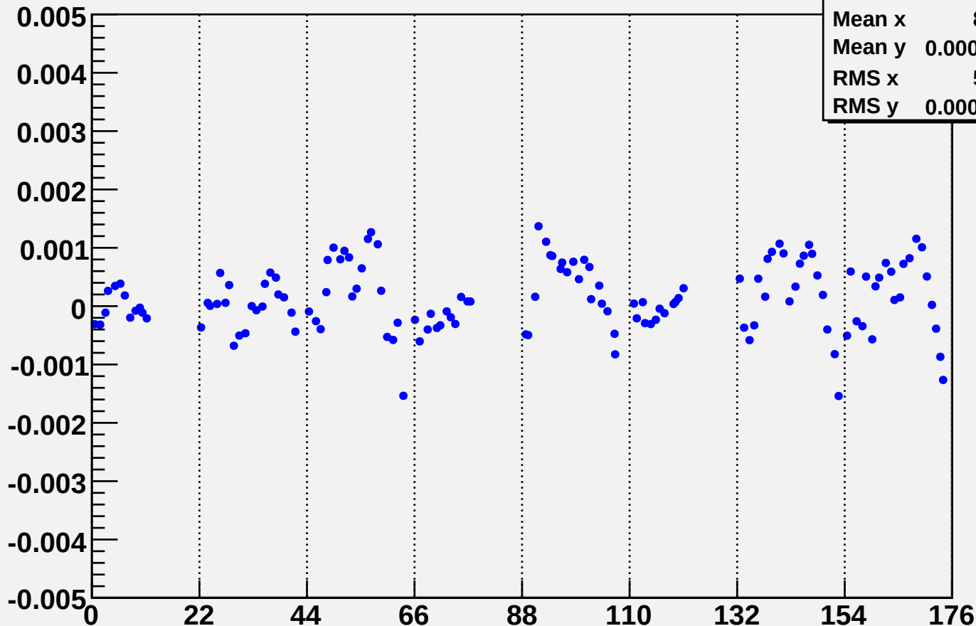
phi residuals vs. hits in ATs
