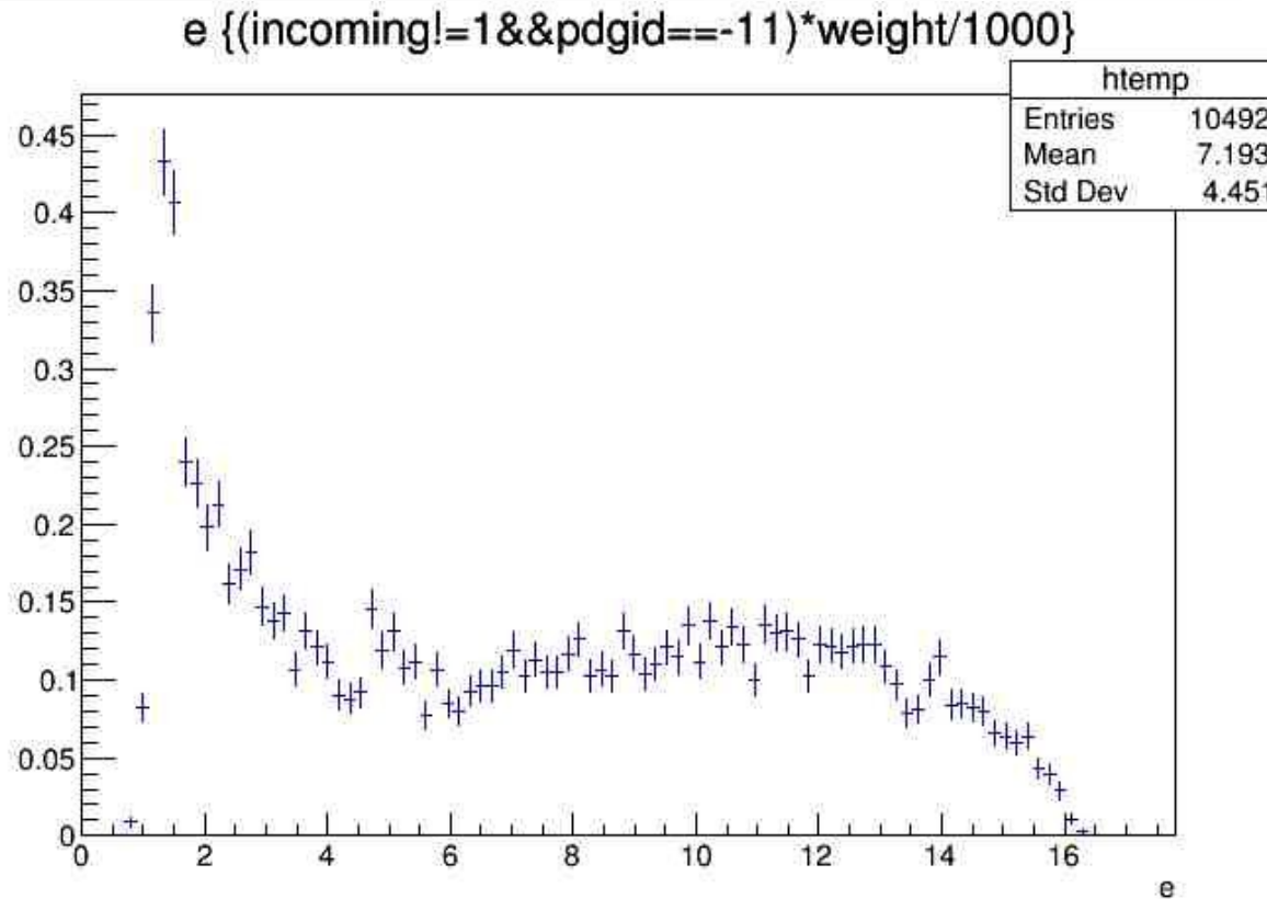
Energy spectrum
