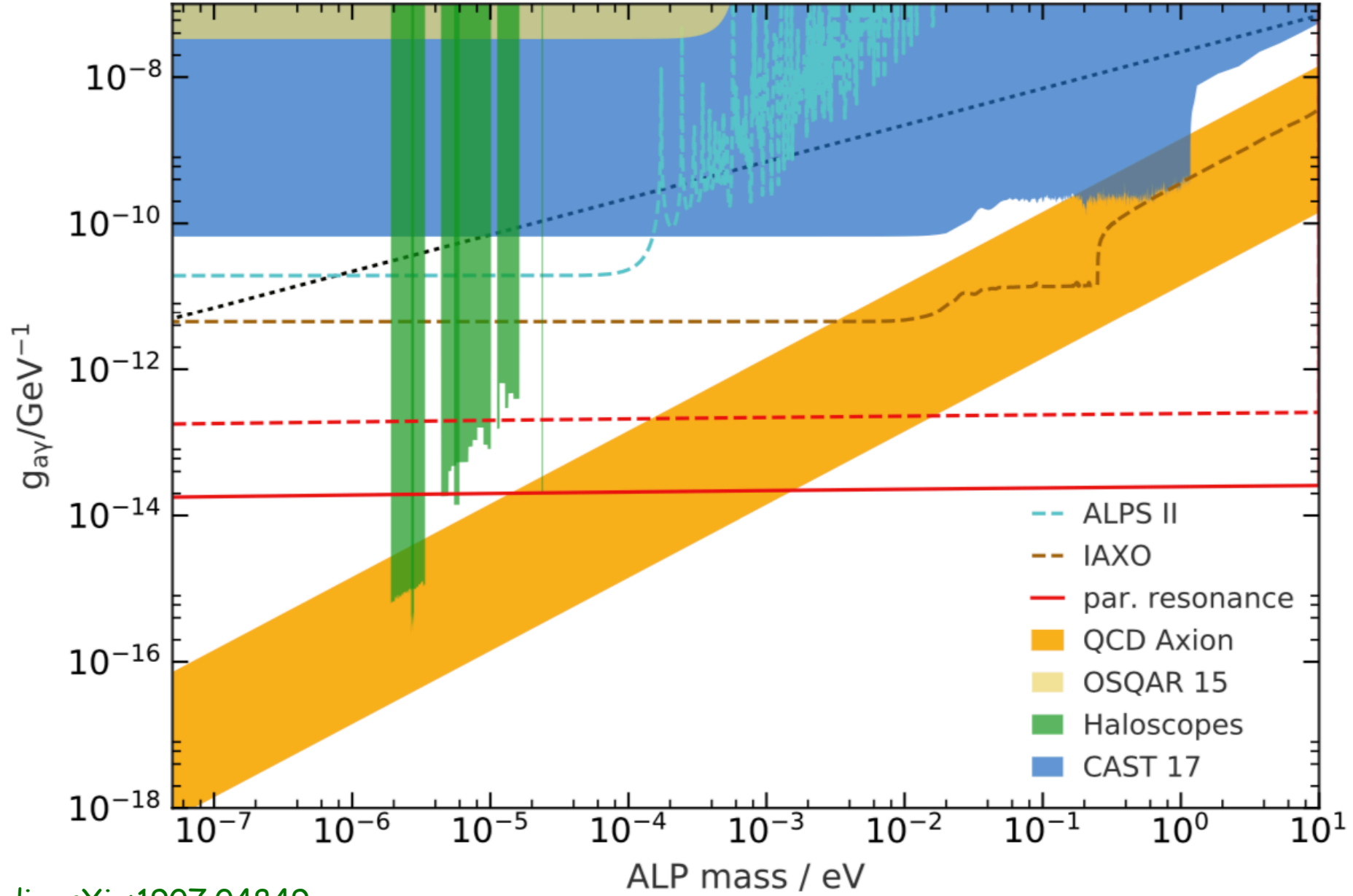
FIG. 1. Axion-photon coupling constant g_{a\gamma} as a function of ALP mass m_a . The red curves depict the constraint from parametric resonance due to axion condensate Galactic dark matter derived from Eq. (9), for R = 10 kpc (solid) and for R = 1 kpc (dashed). Resonant enhancement f \sim 1 and relative channel bandwidth \Delta\nu/\nu \sim 1 are assumed. The constraint on g_{a\gamma} scales logarithmically with m_a (and logarithmically with f\Delta\nu/\nu , if they vary). For comparison, excluded (filled) regions and forecasts (dashed lines) are shown from helioscope, haloscope and light-shining-through-walls experiments. The allowed parameter space for temperature-dependent ALP cold dark matter via the misalignment mechanism [28] is the region below the dotted black line. The orange parallel band depicts QCD axion models [29–32].
