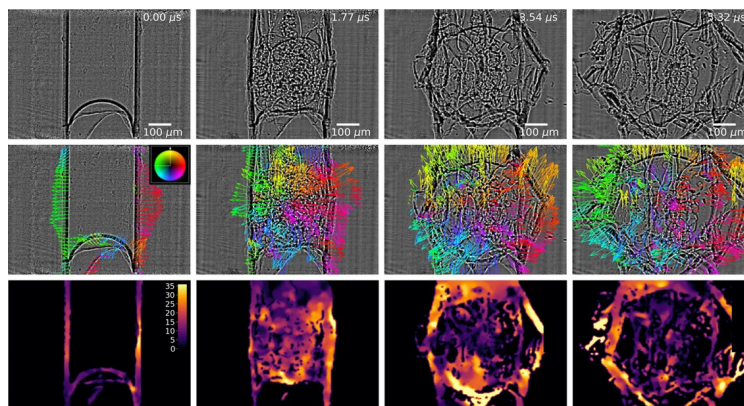
Figure 1: X-ray sequence of laser-induced dynamics in water filled glass capillary imaged at 1.13 MHz sampling rate (top) and processed velocity vectors (middle) and velocities (bottom).
