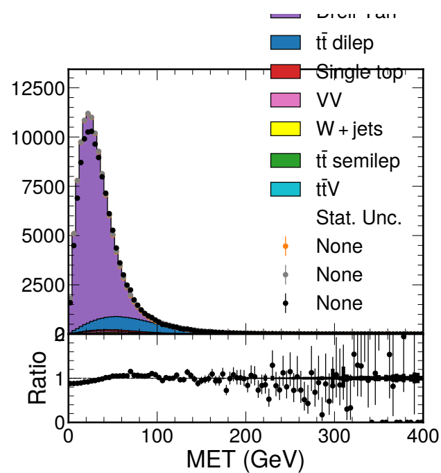
M_{ll} + Z window cuts
