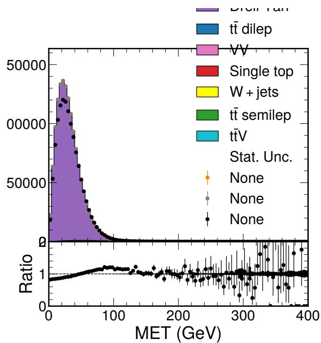
After Triggers + 2 lepton cut
