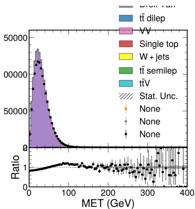
All lepton cuts
