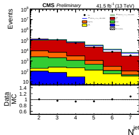
jet multiplicity
