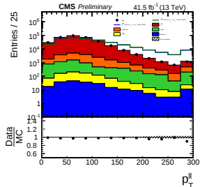
dilepton pt
