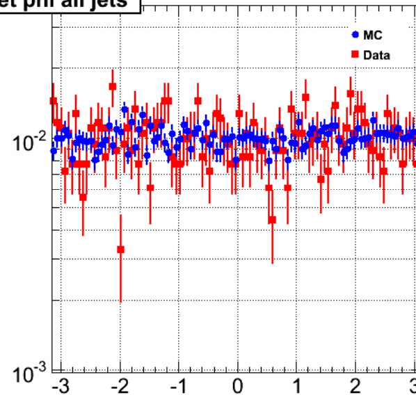
jet phi all jets
