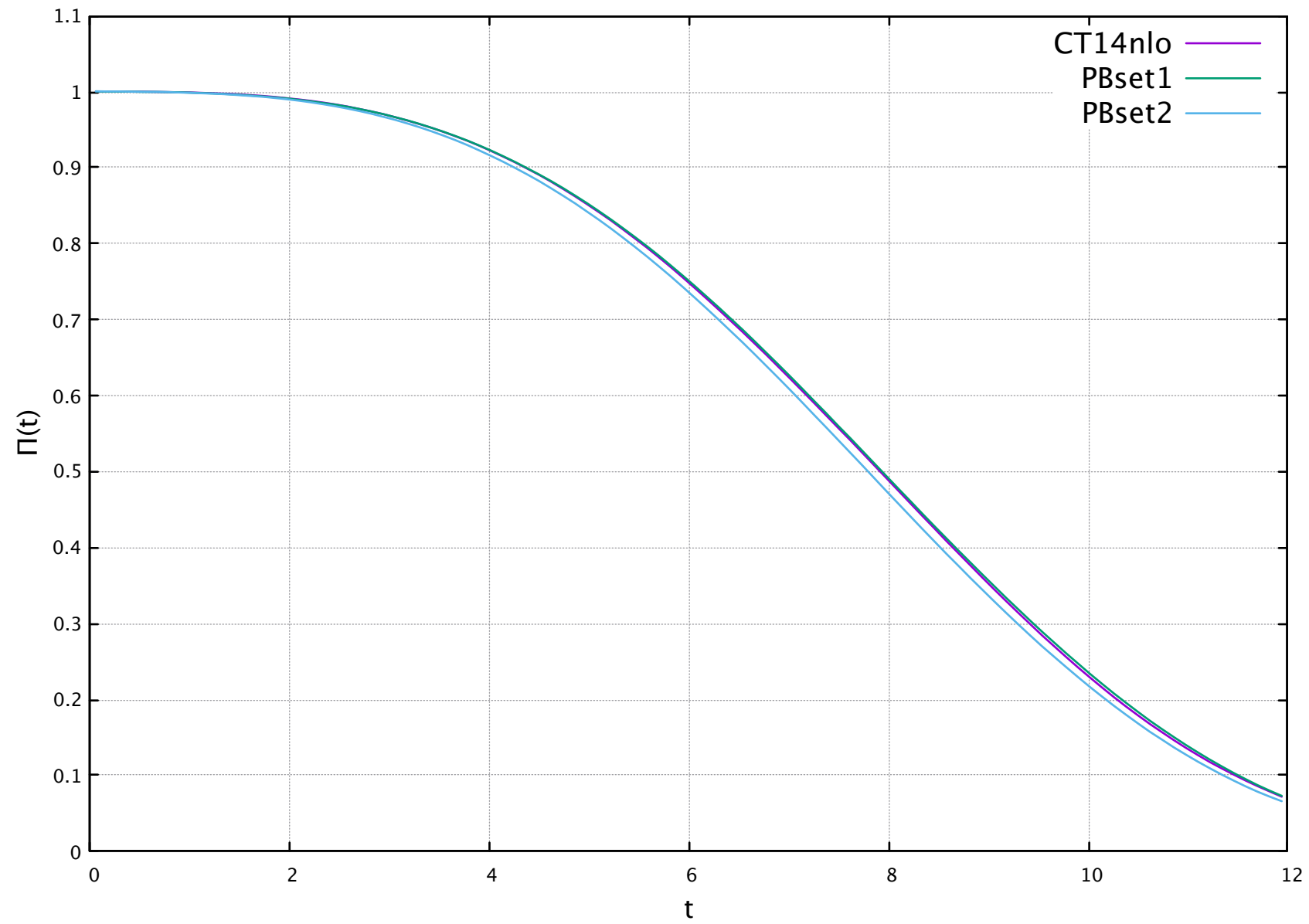
No-emission probability, Pythia
