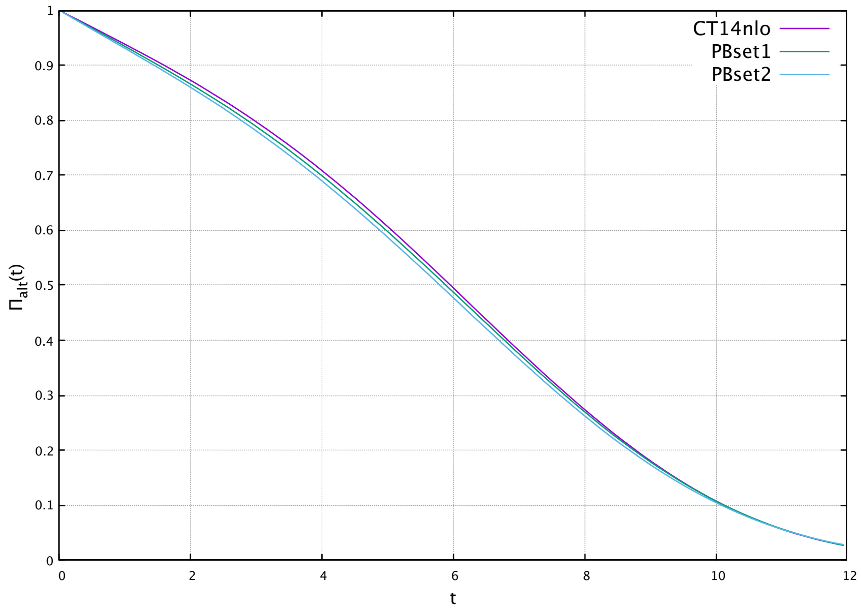
Alternative no-emission probability, Pythia
