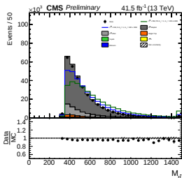
m_ttbar Sonnenschein, DY fxfx
