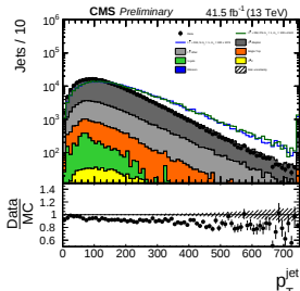
top pt Sonnenschein, DY fxfx, mumu-channel
