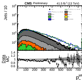
top pt Sonnenschein, DY fxfx, emu-channel
