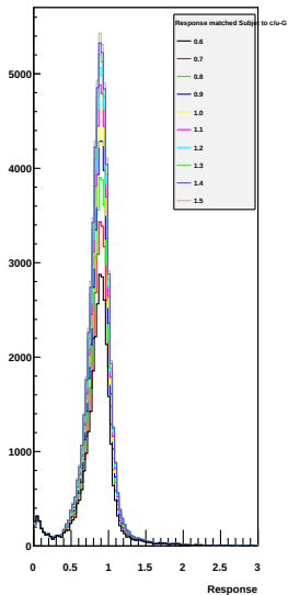
Response Subjet 2/3 to Genparticle
