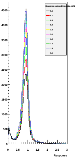
Response Subjet 1/3 to Genparticle
