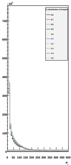
GenJets vs P_t
