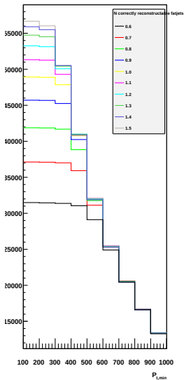
correctly counted, binned in P_{t,min}
