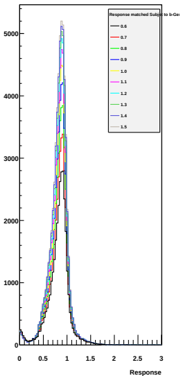
Response b-Subjet to Genparticle
