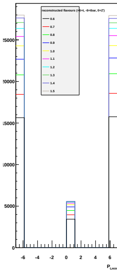
reconstructed flavours ( Z=0 , t=6 , tbar=6 )
