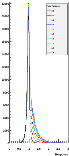
Response Fatjet to Genjet
