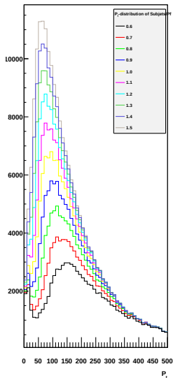
SubJets vs P_{t,t}
