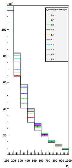
FatJets vs P_t
