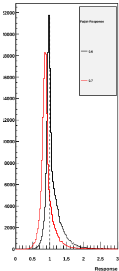
Response Fatjet to Genjet
