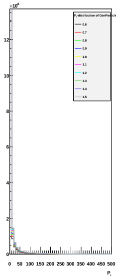
GenParticles vs P_{t,t}
