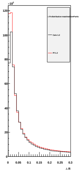
dR of matched GenParticles to SubJets
