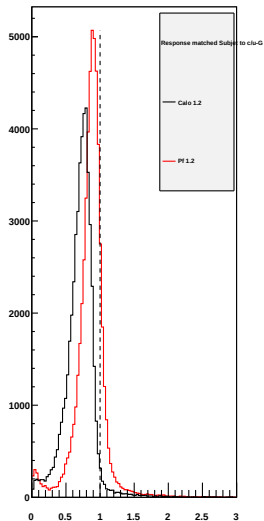
Response Subjet 2/3 to Genparticle
