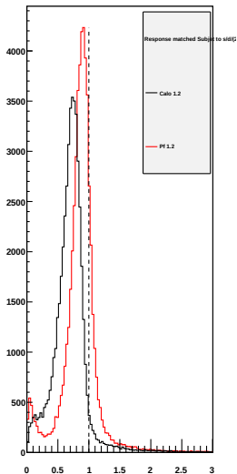
Response Subjet 1/3 to Genparticle
