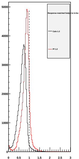
Response b-Subjet to Genparticle
