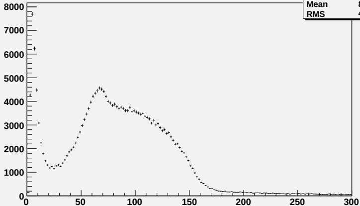
all subjects of single fatjets invariant mass
