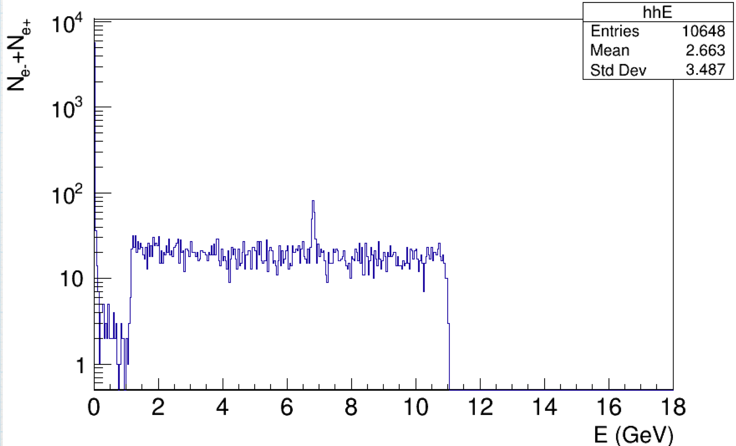
Energy spectrum
