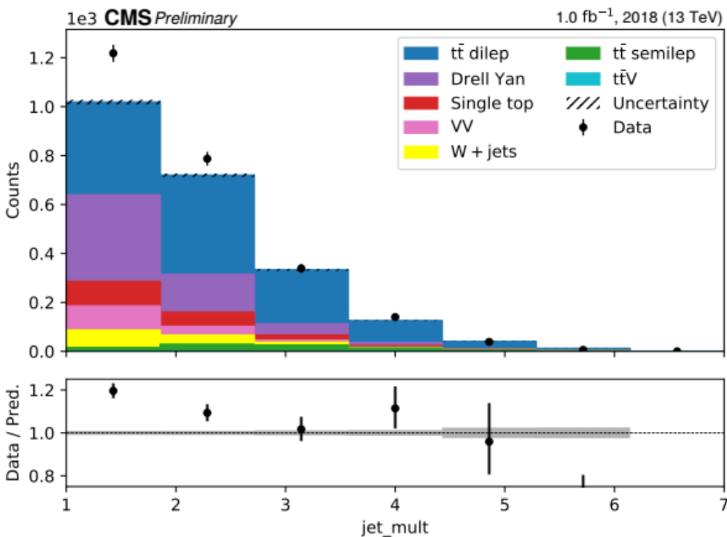
Deep Jet
