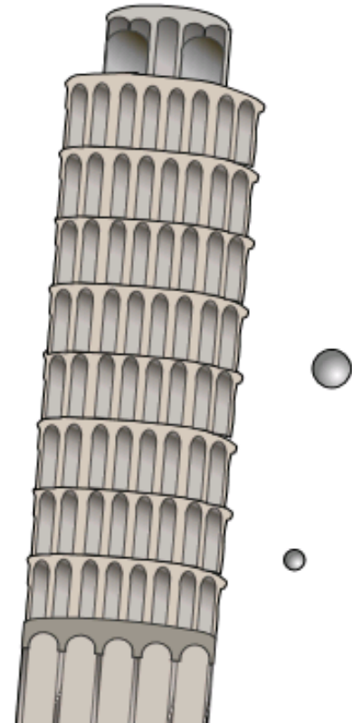
Dark Energy?
