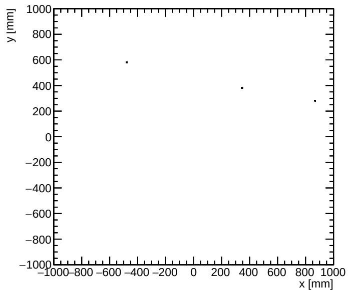
muons+ detector y vs x for E > 0.5 GeV
