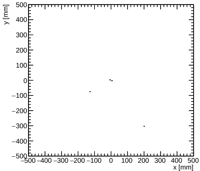
numubar vertex y vs x for E > 0.5 GeV
