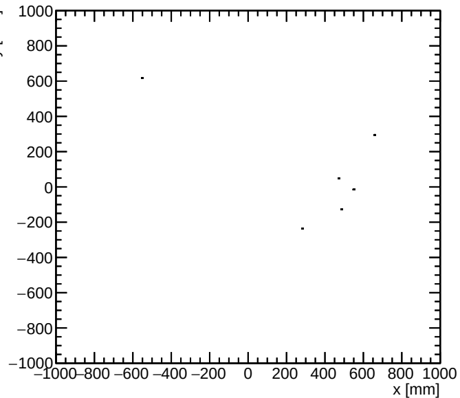
kaon- detector y vs x for E > 0.5 GeV
