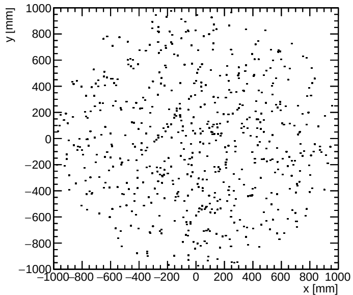
neutrons detector y vs x for E > 0.5 GeV
