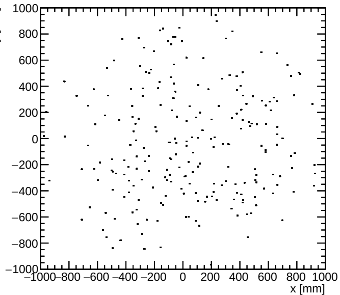
protons- detector y vs x for E > 0.5 GeV
