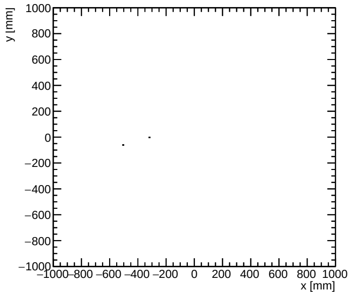
kaon- detector y vs x for E > 0.5 GeV
