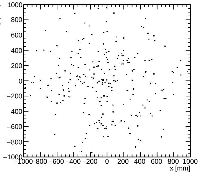
pions+ detector y vs x for E > 0.5 GeV
