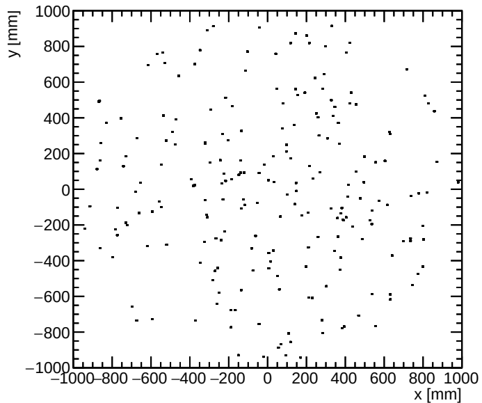
protons- detector y vs x for E > 0.5 GeV
