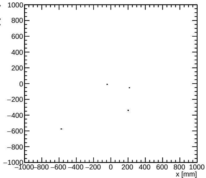
numubar detector y vs x for E > 0.5 GeV
