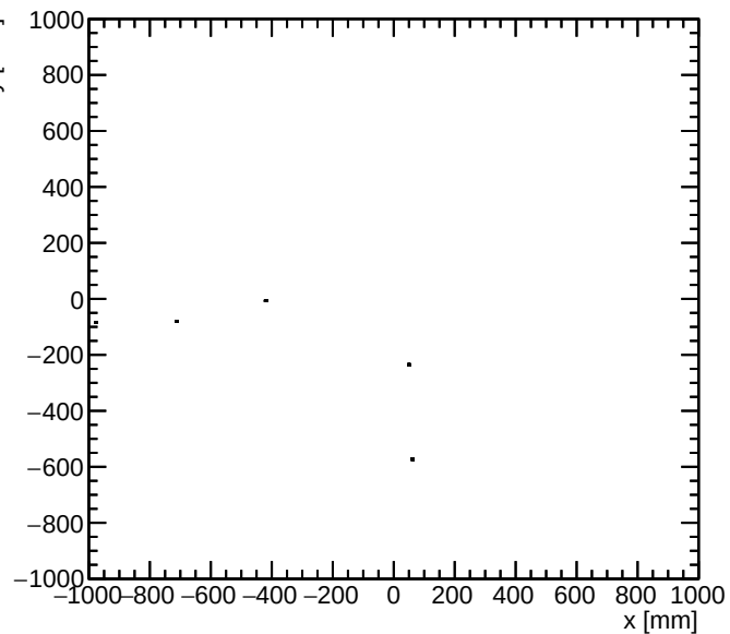
numu detector y vs x for E > 0.5 GeV
