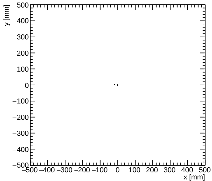
kaon0L vertex y vs x for E > 0.5 GeV
