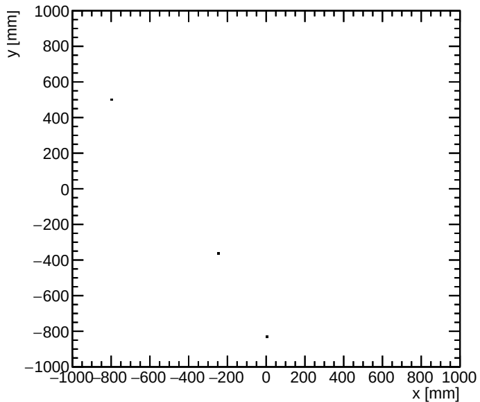
numubar detector y vs x for E > 0.5 GeV
