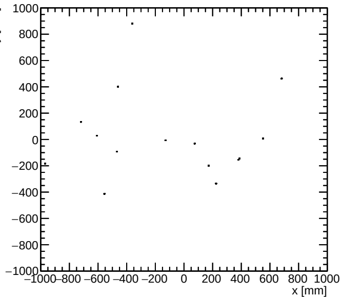
muons- detector y vs x for E > 0.5 GeV
