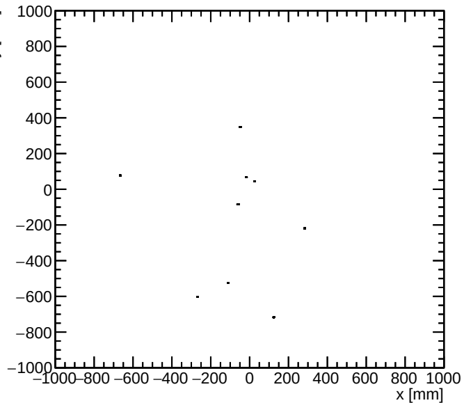
kaon0L detector y vs x for E > 0.5 GeV
