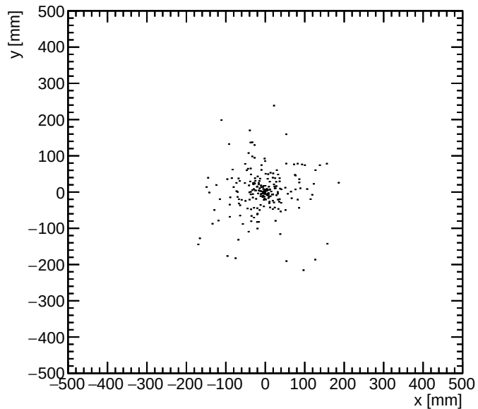
neutrons vertex y vs x for E > 0.5 GeV
