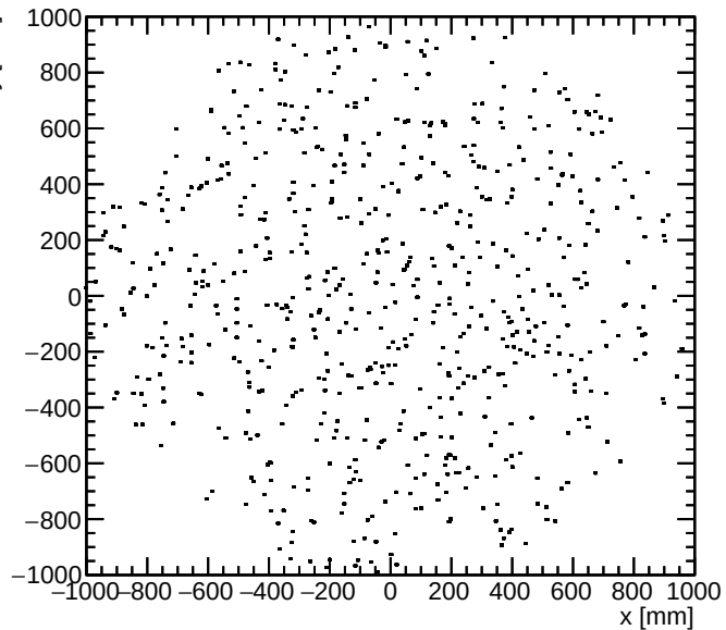
neutrons detector y vs x for E > 0.5 GeV
