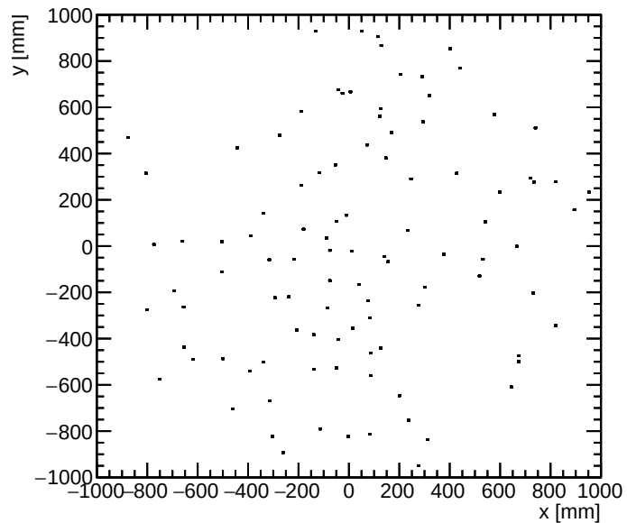
pions- detector y vs x for E > 0.5 GeV
