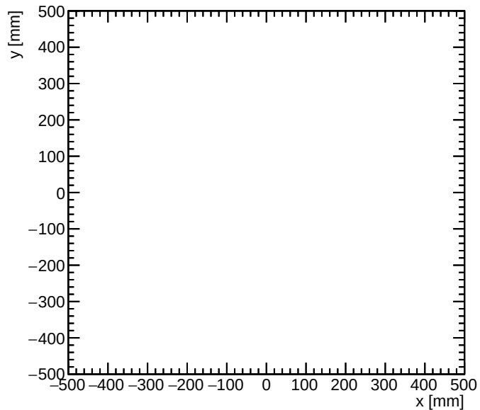
photons vertex y vs x for E > 0.5 GeV
