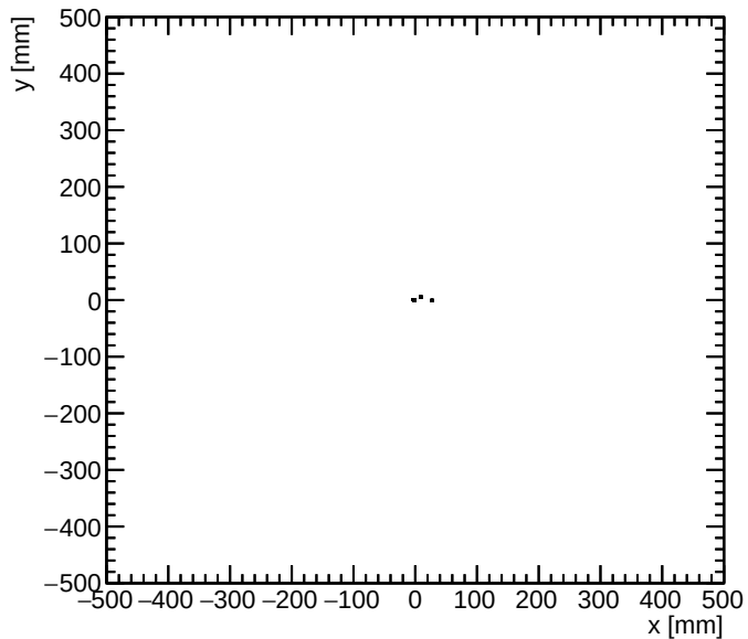
kaon- vertex y vs x for E > 0.5 GeV
