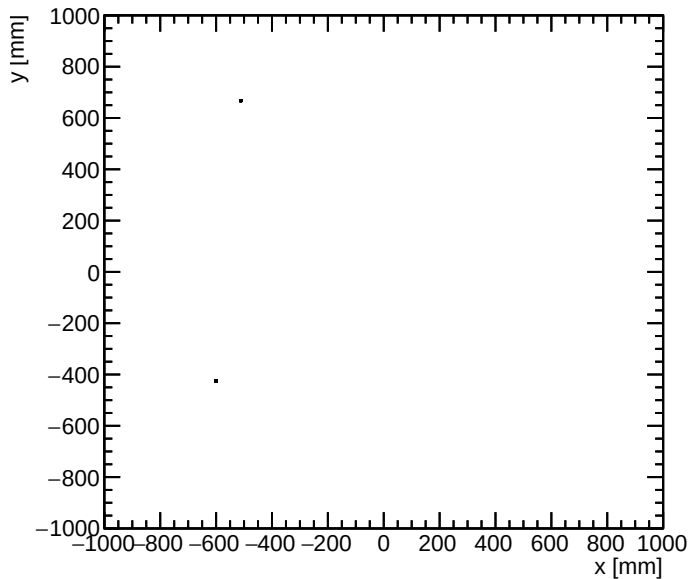
kaon0L detector y vs x for E > 0.5 GeV
