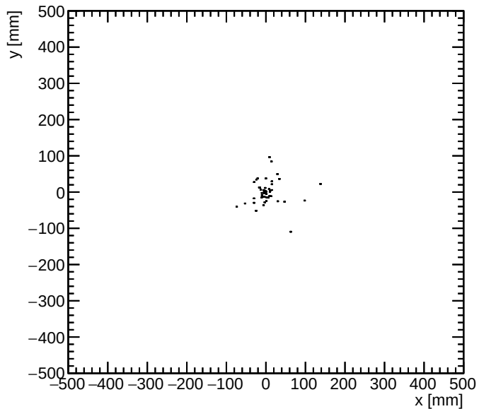
pions- vertex y vs x for E > 0.5 GeV
