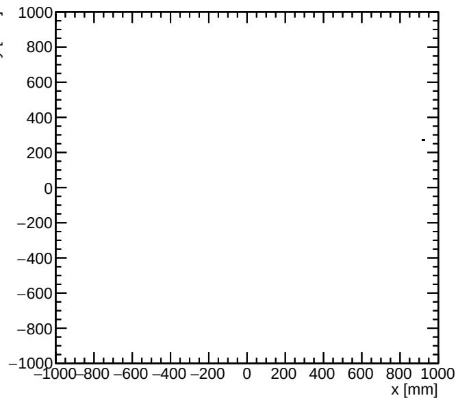
deuteron detector y vs x for E > 0.5 GeV
