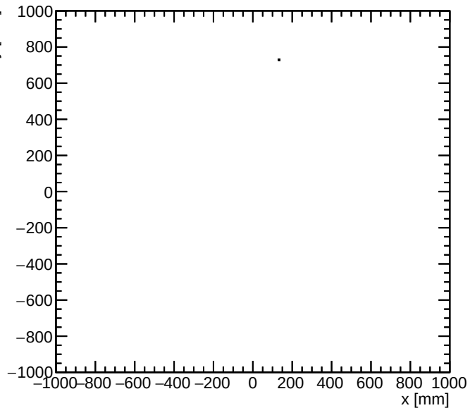
neutronsbar detector y vs x for E > 0.5 GeV
