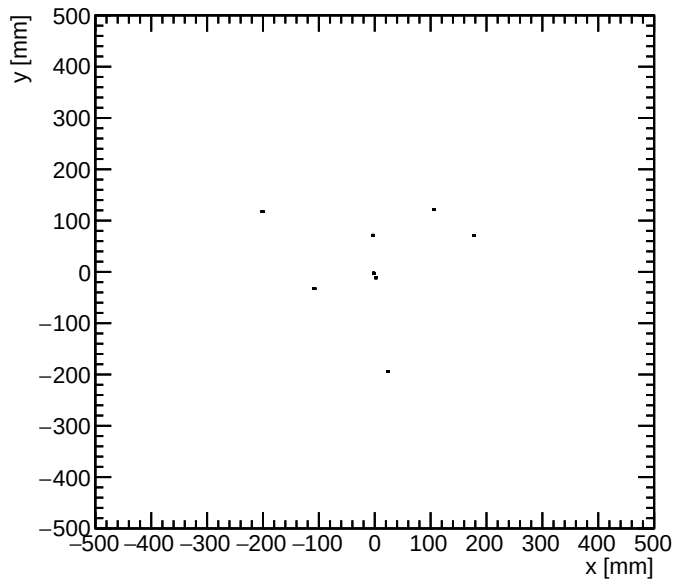
muons- vertex y vs x for E > 0.5 GeV
