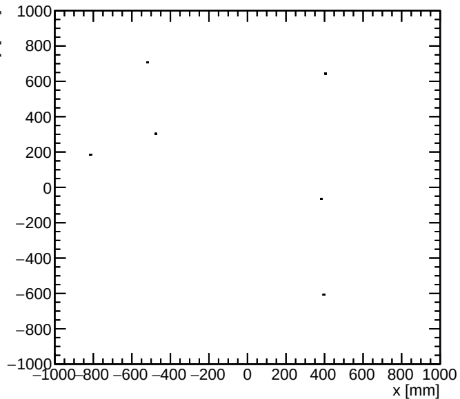
photons detector y vs x for E > 0.5 GeV
