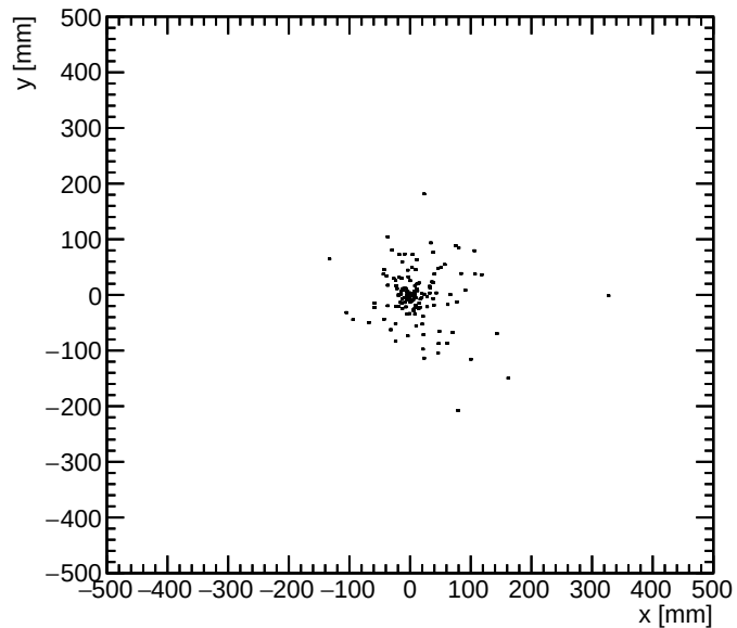
protons- vertex y vs x for E > 0.5 GeV
