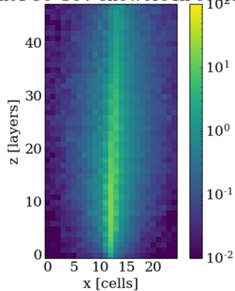
Geant4 50 GeV showers4k overlay
