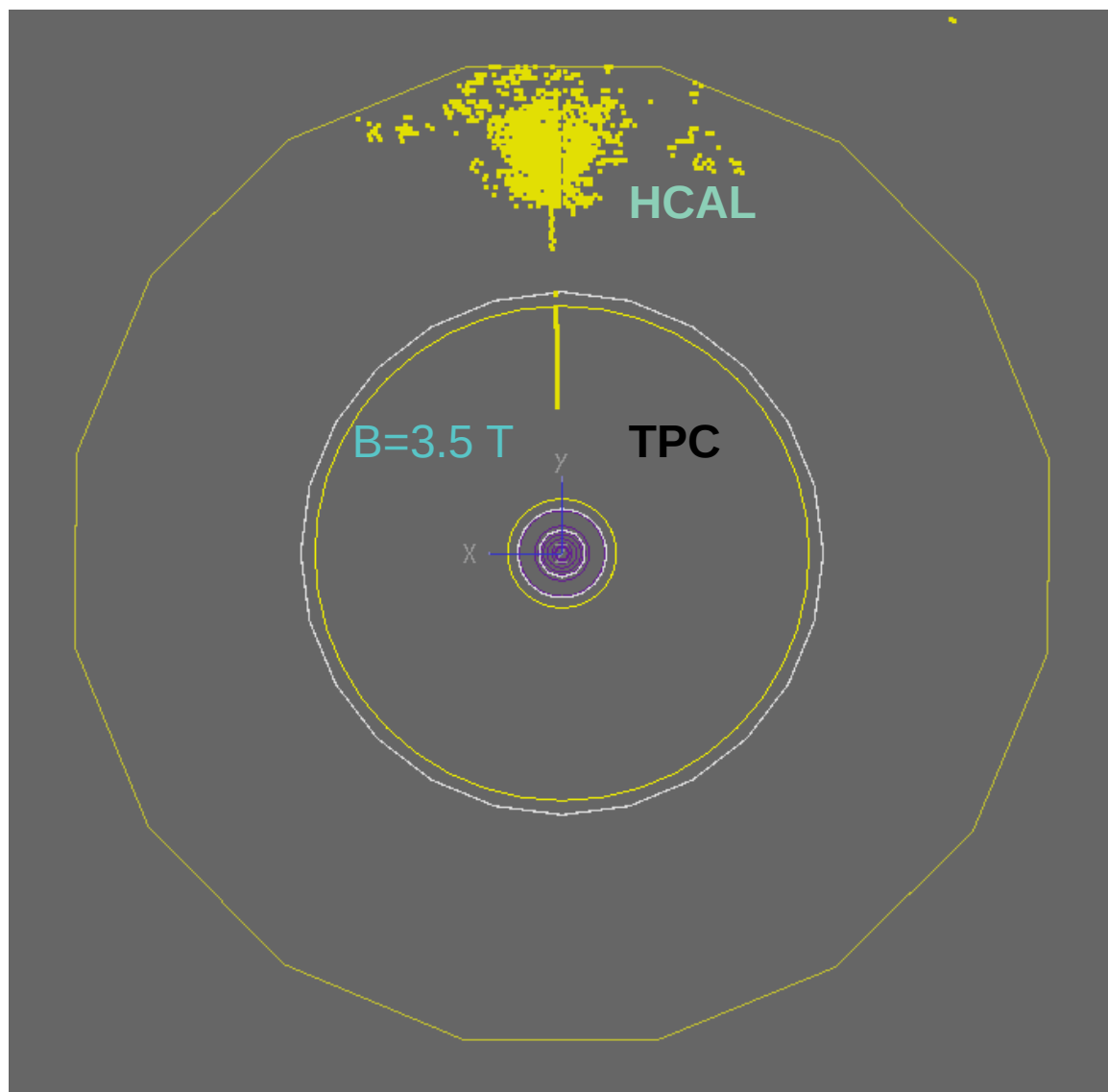
Example event: 30 GeV pion
