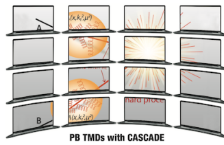
PB TMDs with CASCADE
