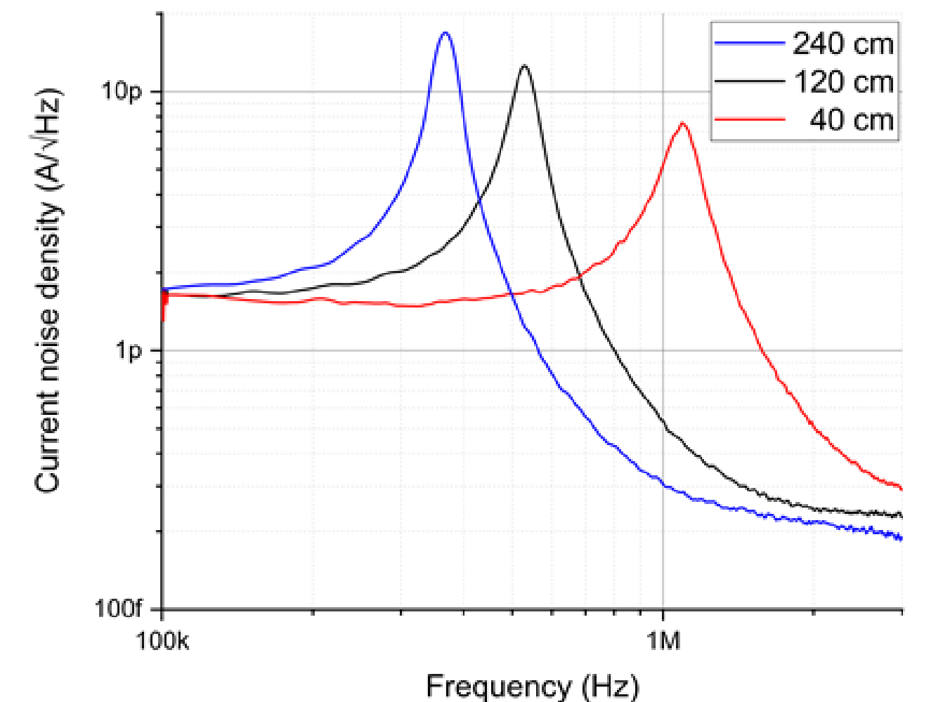
Figure 6: LC-resonance peaks of the DCCC at three processing stages with increasing number of meander pairs or effective length of the shielding tube package.
