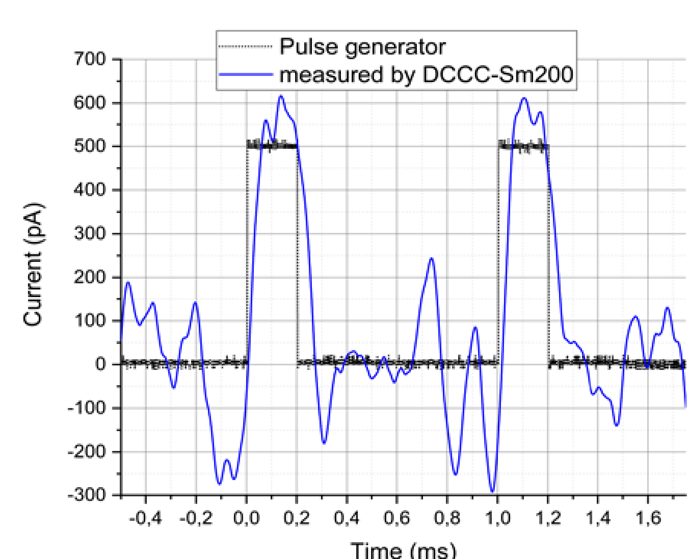
Figure 8: Pulse current resolution of the final DCCC-Sm-200, both pickup coils on one SQUID with input inductance of 1 \mu\text{H} .
