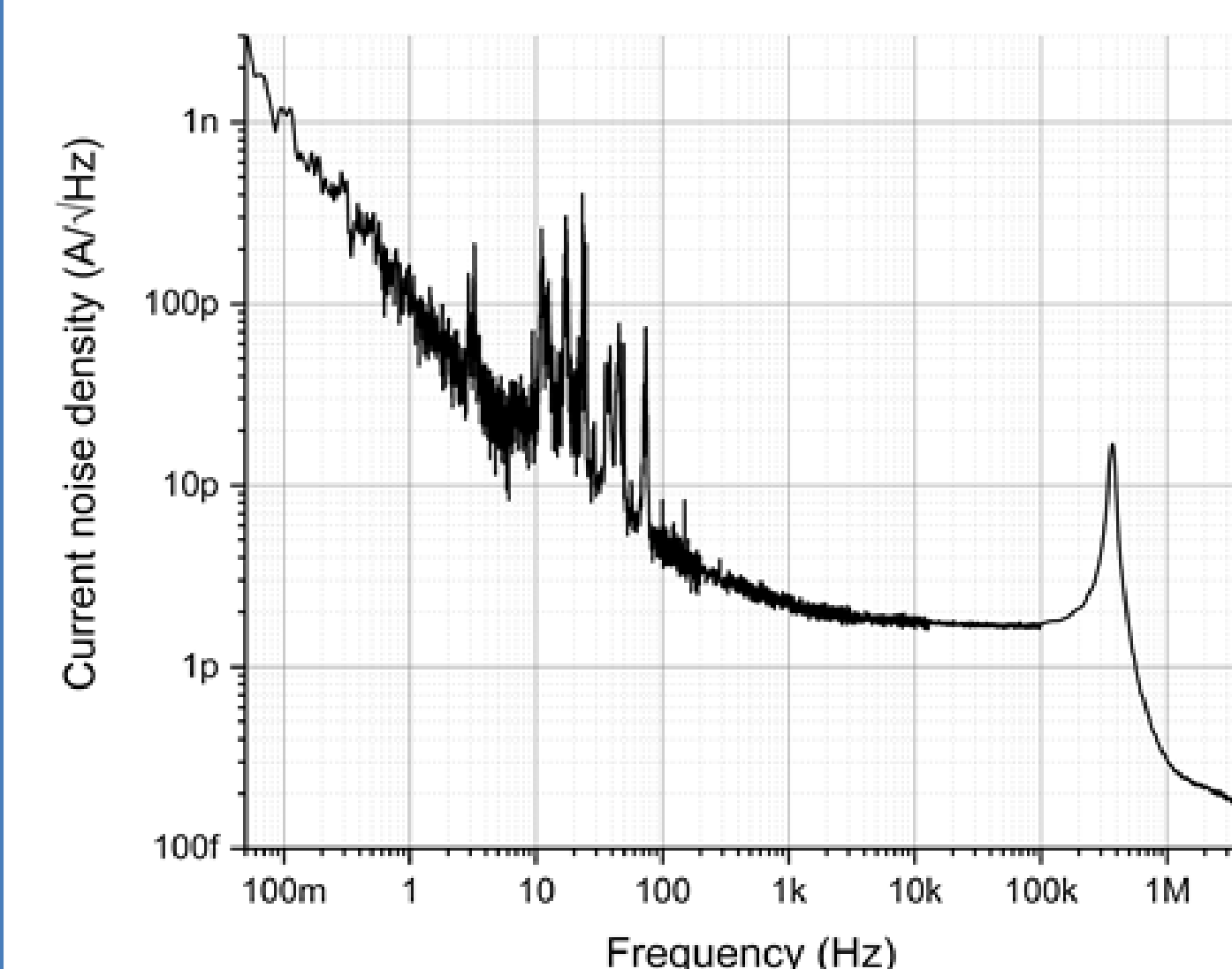
Figure 7: Total current noise density spectrum of the final DCCC-Sm-200, both pickup coils on one SQUID with input inductance of 1 \mu\text{H} .
