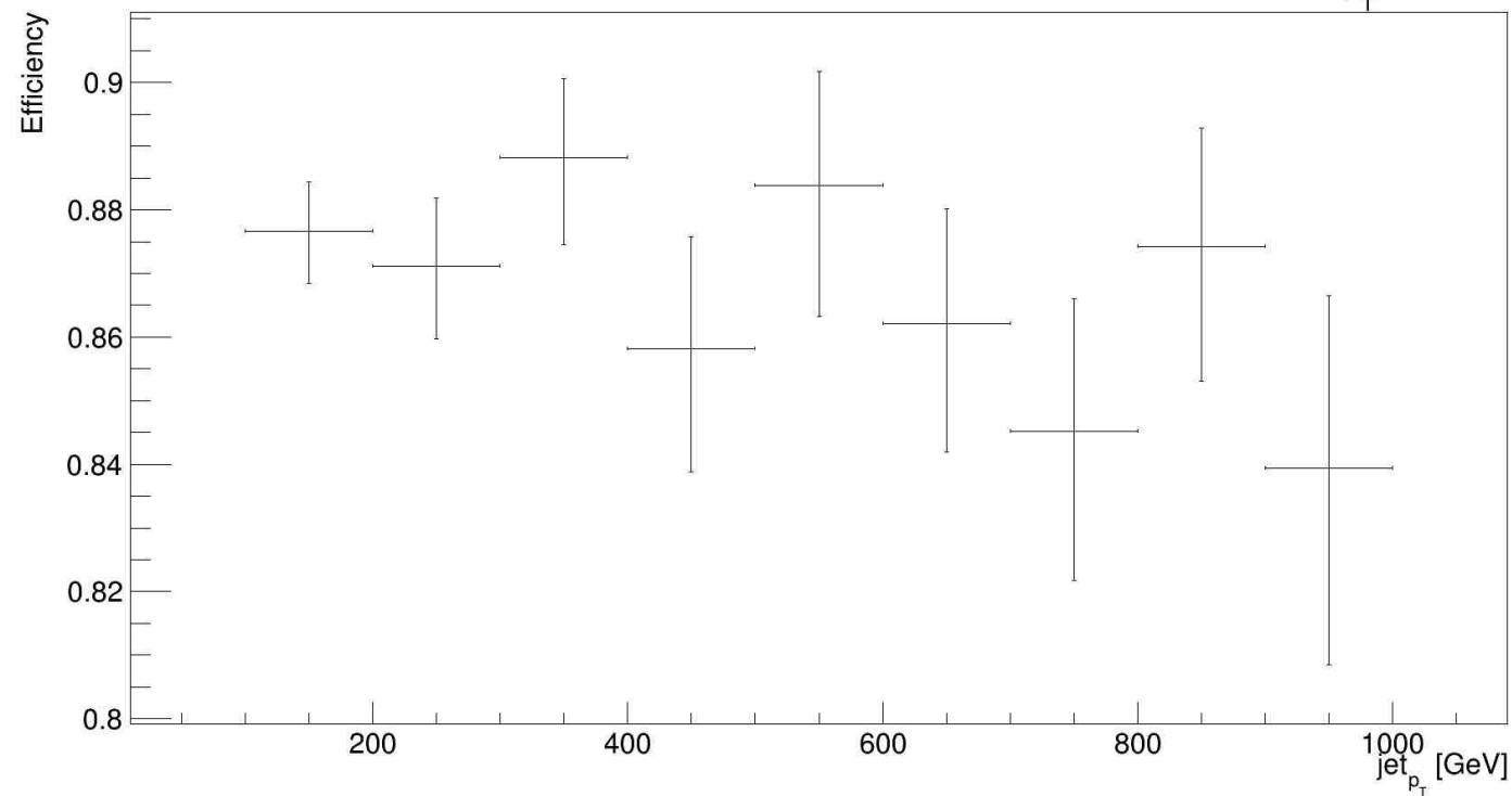
Fraction of reco-matched truth track versus jet p_T
