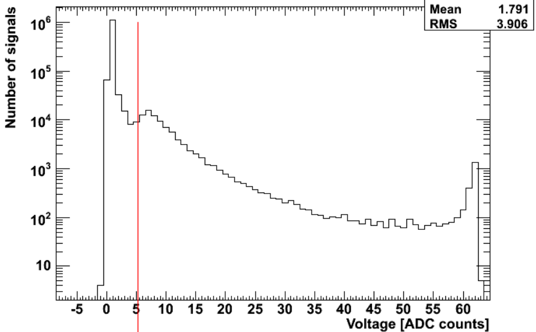
Pulse Height Spectrum (pedestal not scaled)
