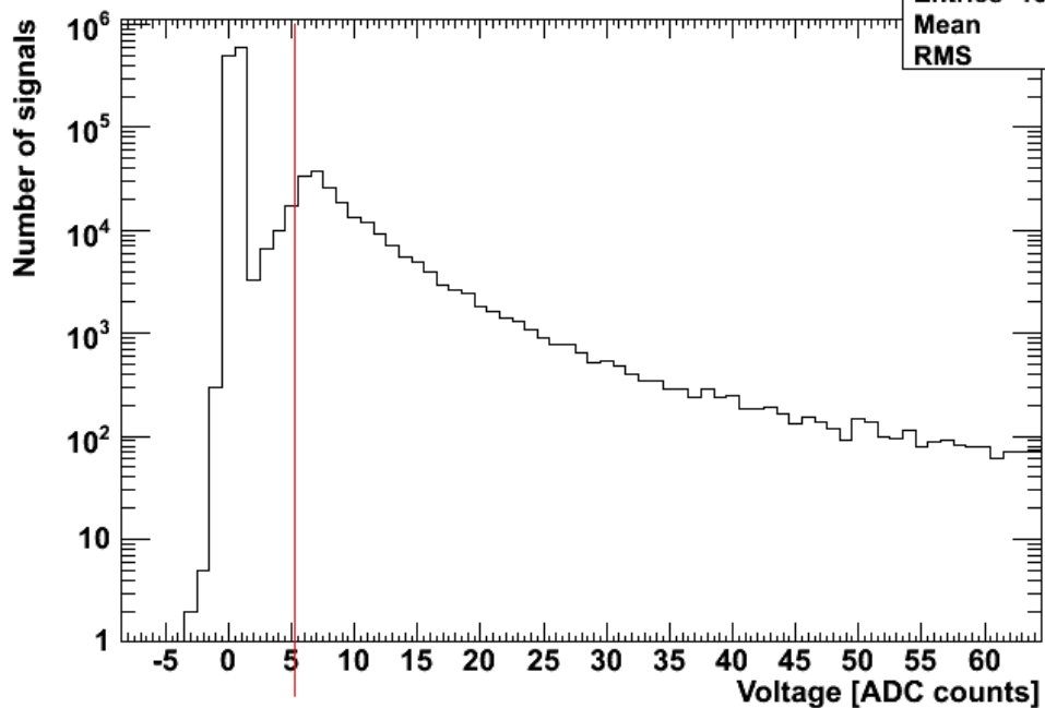
Pulse Height Spectrum (pedestal not scaled)
