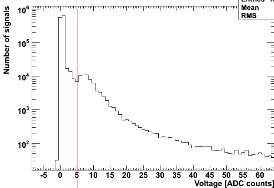
Pulse Height Spectrum (pedestal not scaled)
