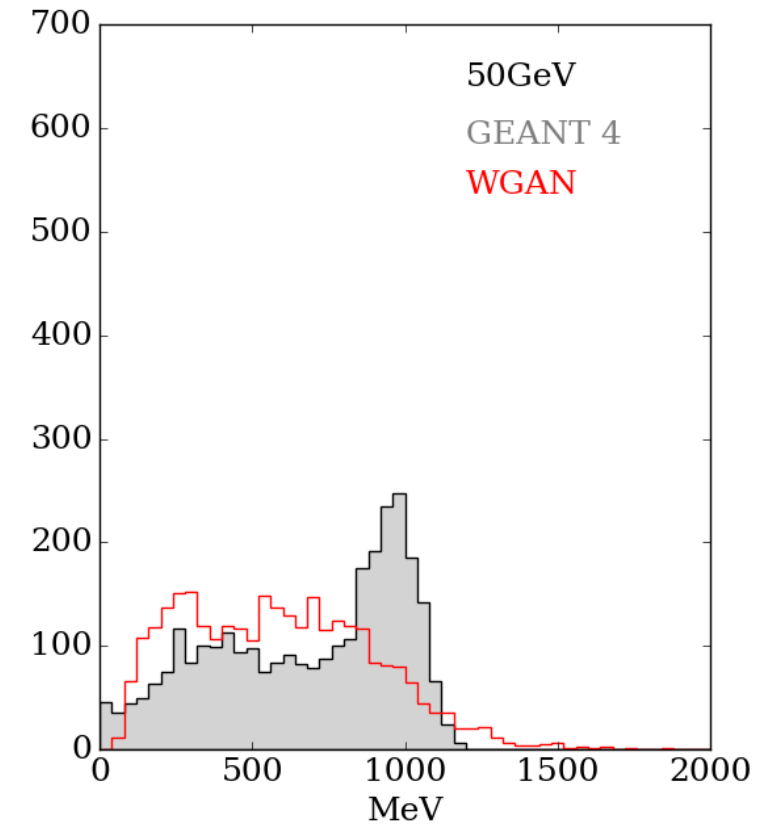
HCAL
