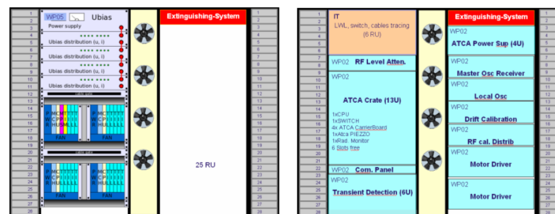
Power coupler / LLRF Cabinet at 712 m
