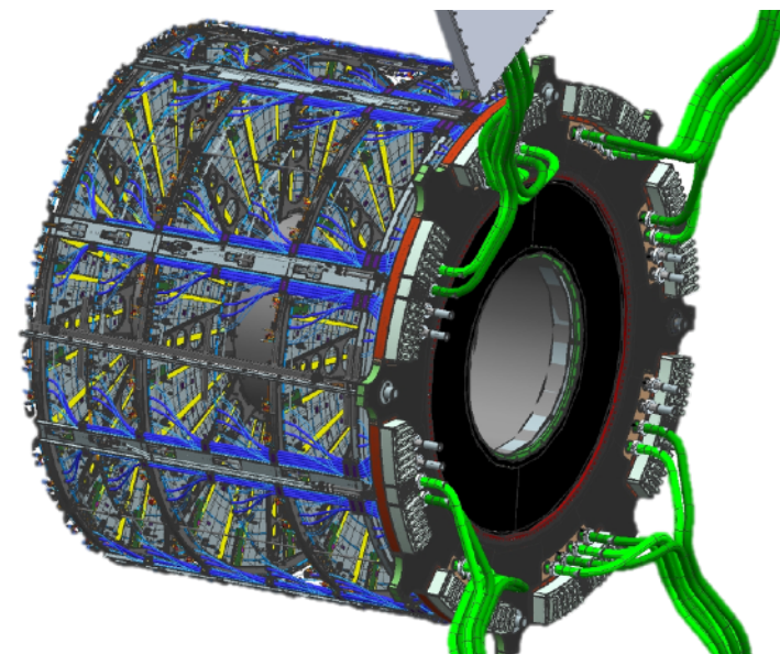
Ready for installation in the ATLAS experiment
