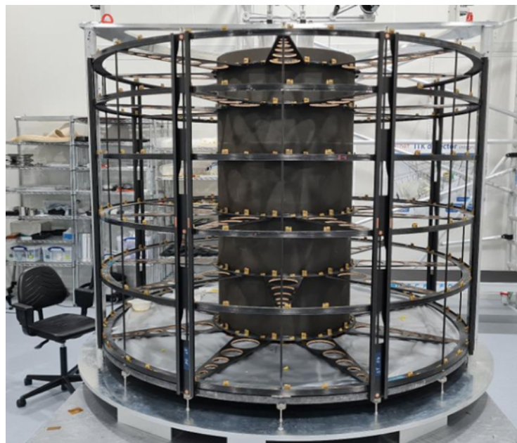
Integrate the petals in the Endcap structure
