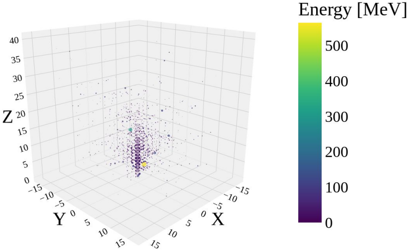
Geant 4
