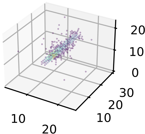
Python JIT
