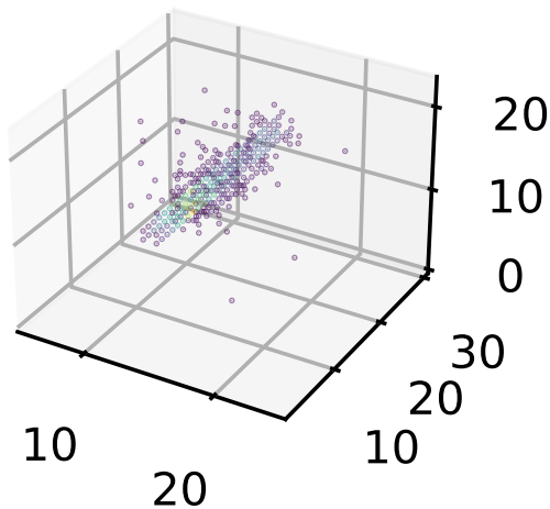
C++ JIT
