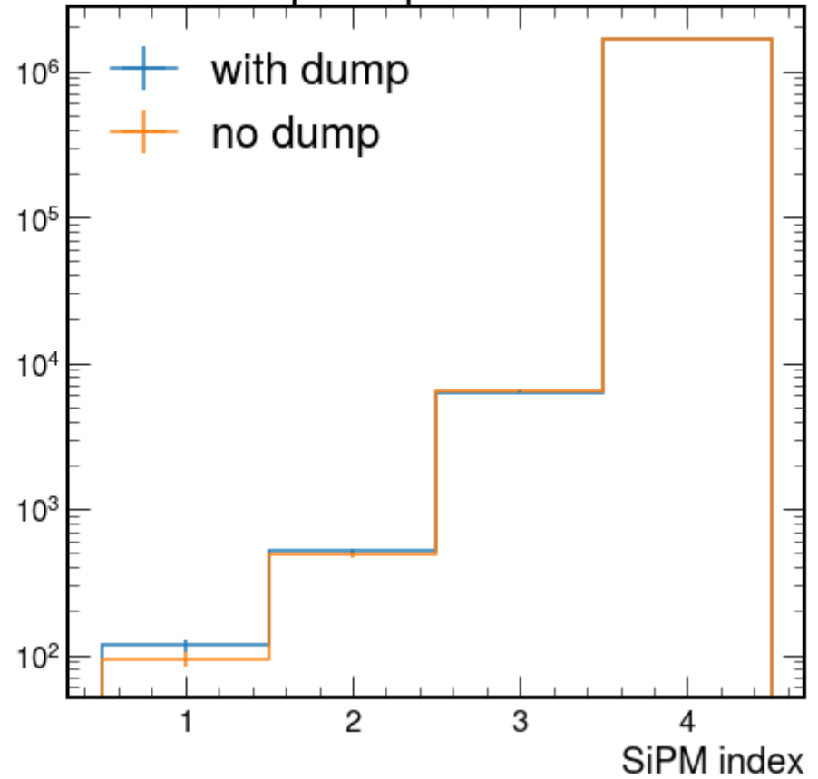
Optical photon hits
