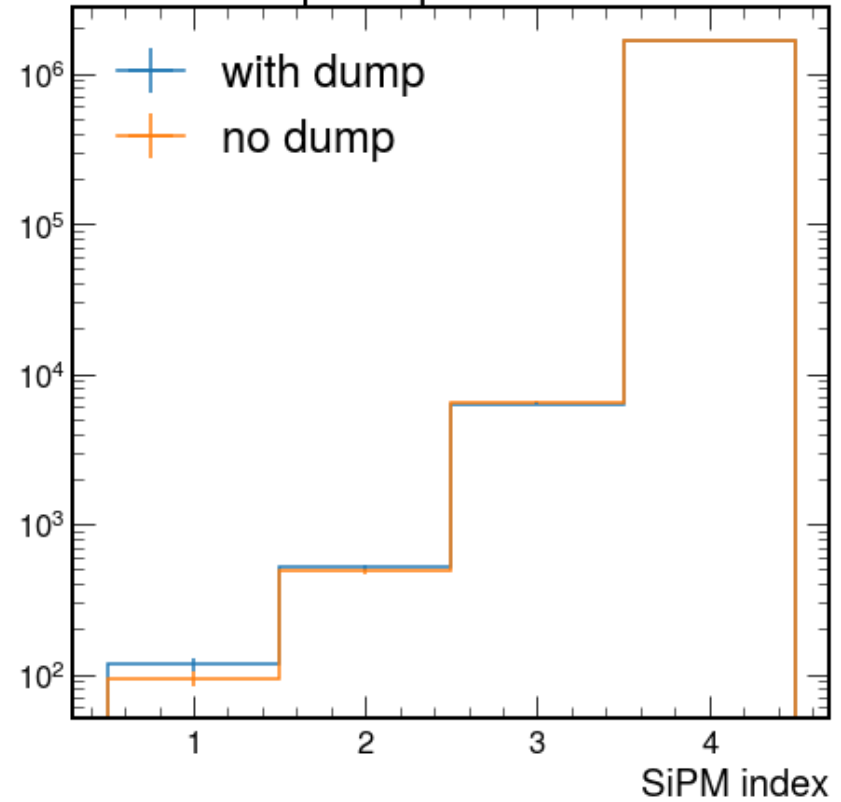
Optical photon hits
