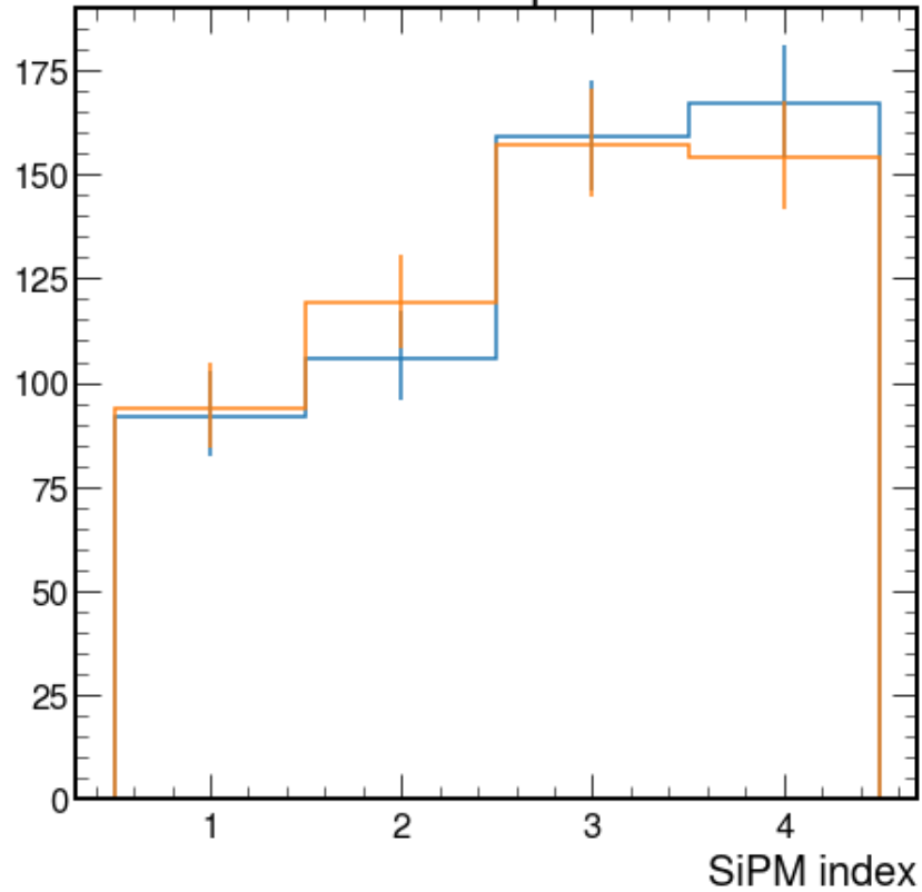
Direct electron/positron hits
