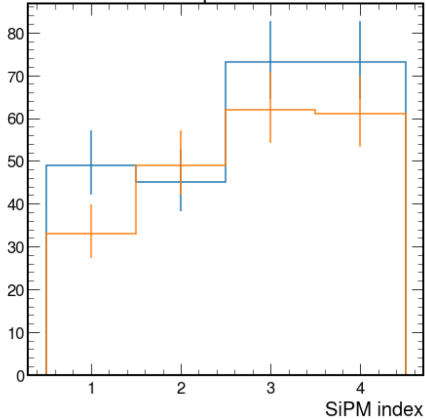
Direct photon hits
