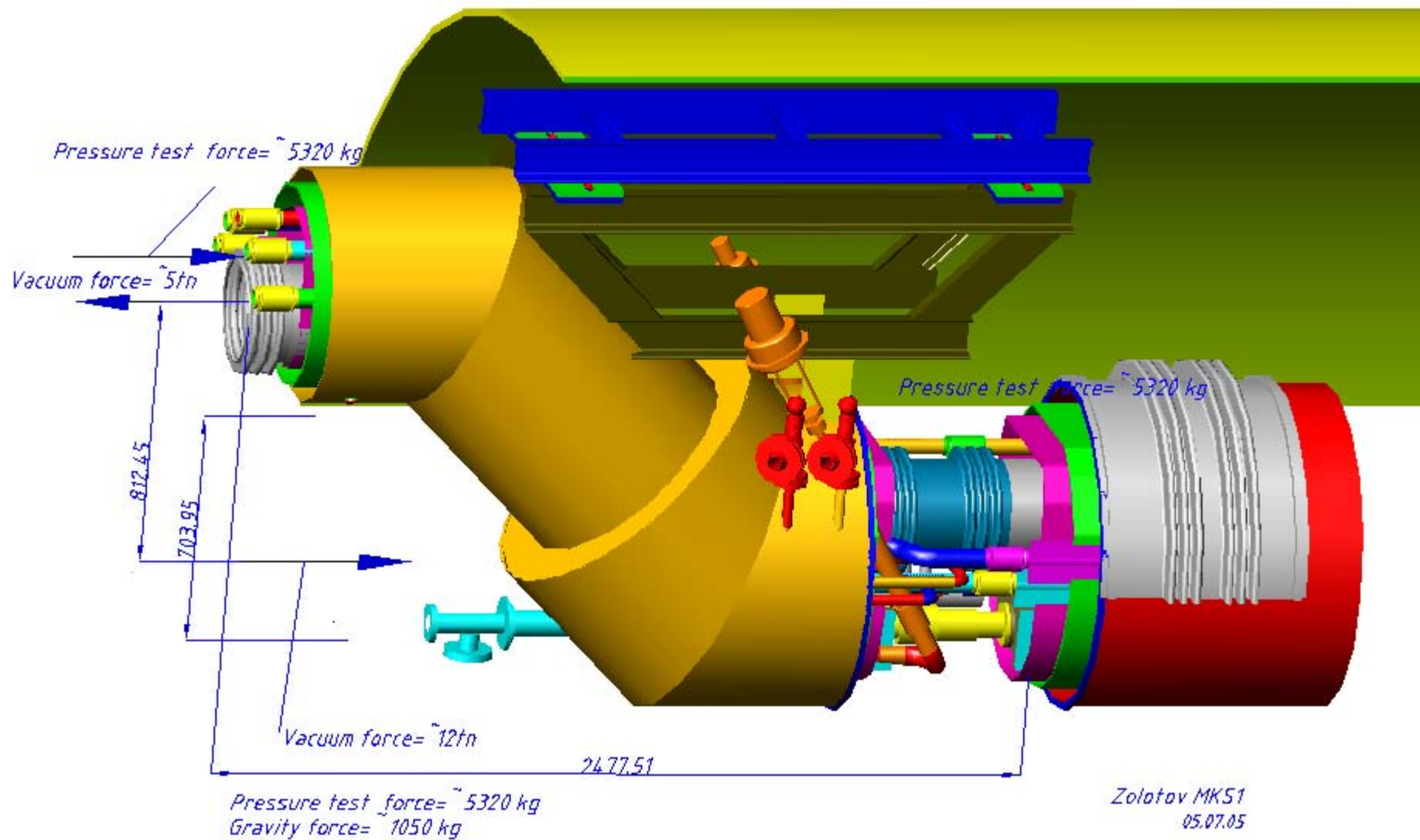
XFEL Feed&turn box
