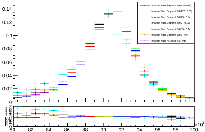
Invariant Mass - All Rings
