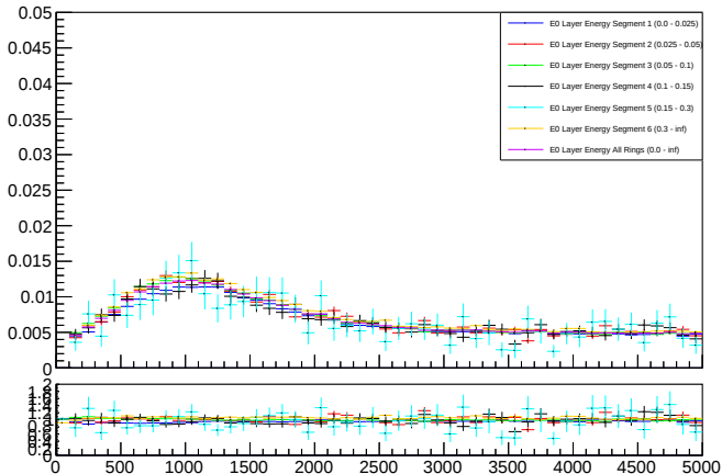
E0 Layer Energy - All Segments
