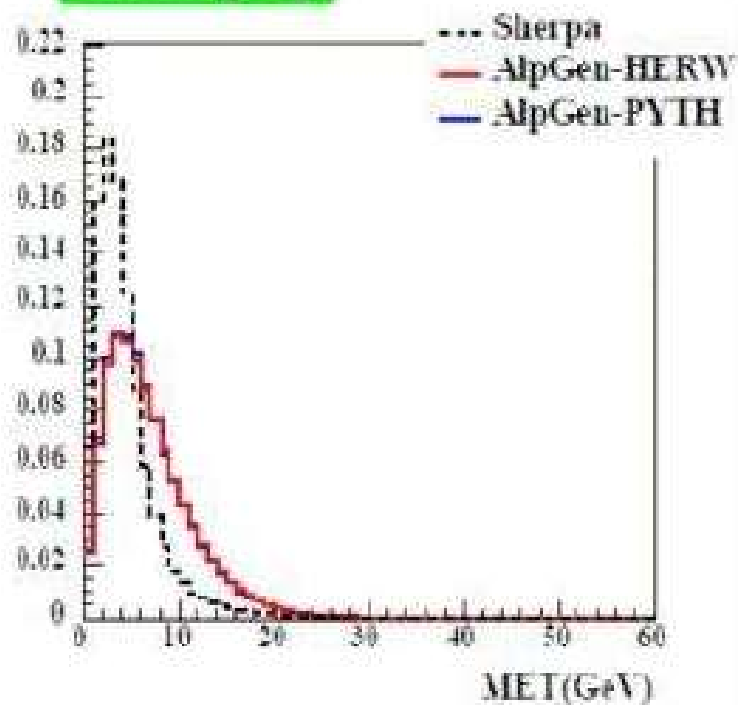
Missing E_T
