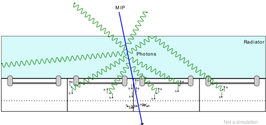
DSiPM + Thin LYSO concept
