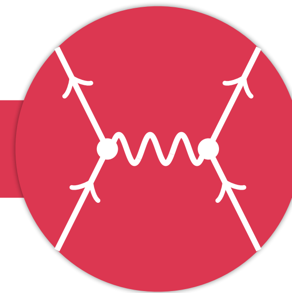
Amplitude Surrogates
