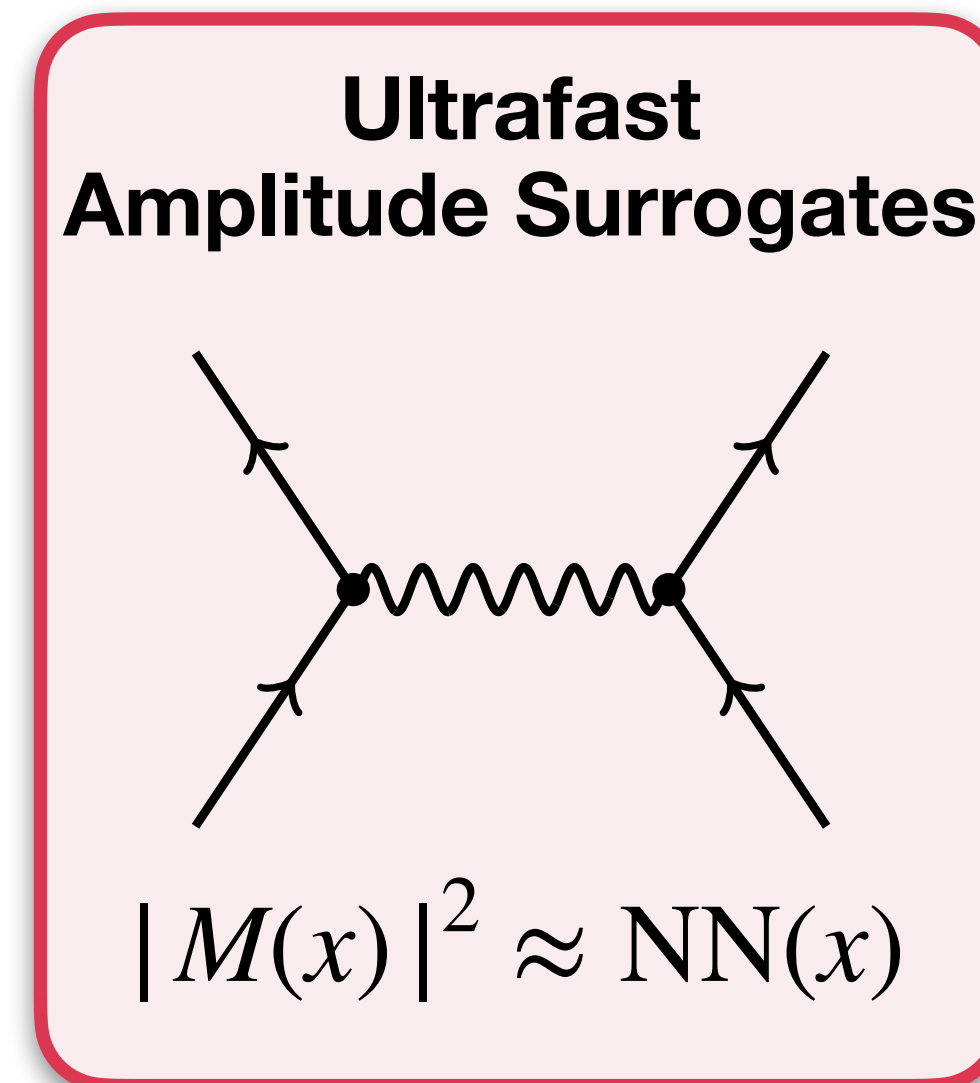
Amplitude Surrogates
