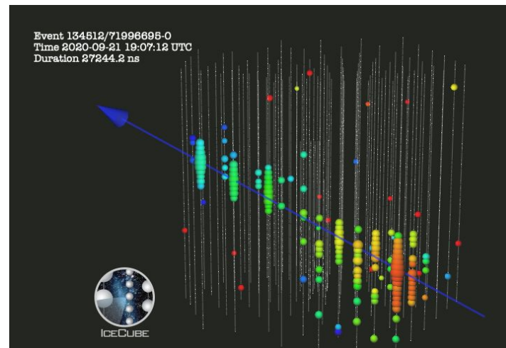
Illustration of a neutrino interaction in the IceCube detector underneath the antarctic ice. Credit: IceCube Collaboration
