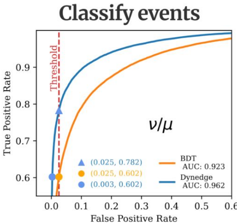
Resolution and ROC curves (blue) of models trained to reconstruct the zenith angle and distinguish between muon and neutrino events . Compared against SOTA (orange). arXiv:2209.03042
