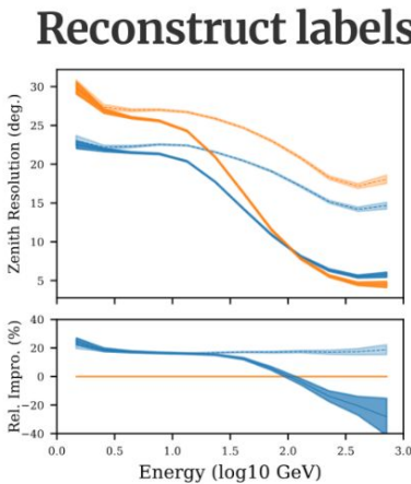
Resolution and ROC curves (blue) of models trained to reconstruct the zenith angle and distinguish between muon and neutrino events . Compared against SOTA (orange). arXiv:2209.03042
