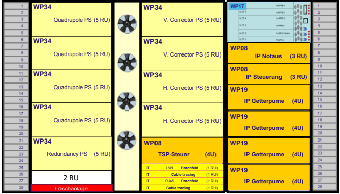
Power supplies
