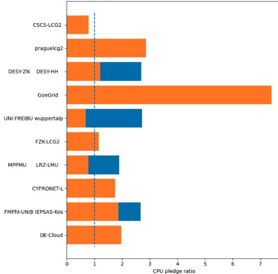
CPU HS06 pledge ratio from 2025-02-01 00:00:00 to 2025-03-01 00:00:00
