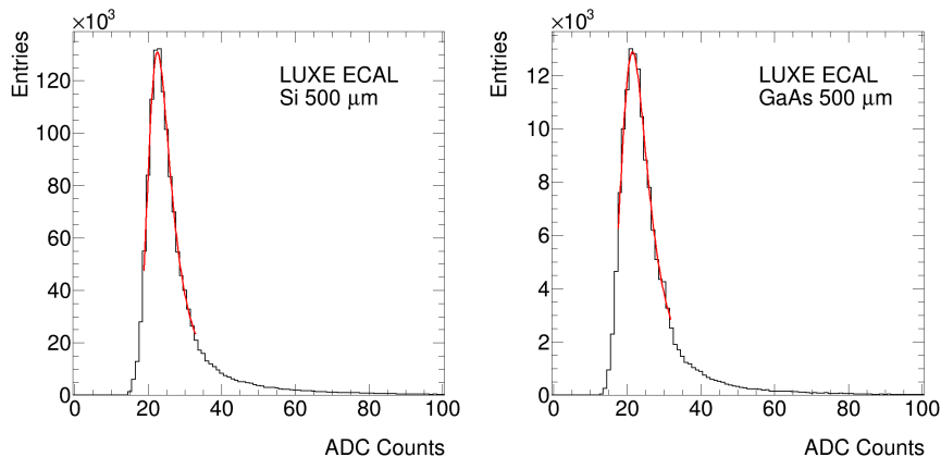
Fig. 16 Distribution of the signal in a pad of the Si (left) and GaAs (right) sensor. The continuous line represents the result of a fit with a Landau distribution function convoluted with a Gaussian in the corresponding range.
