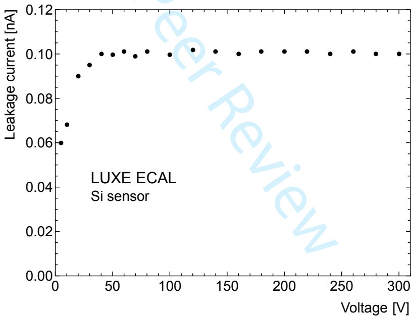
Fig. 2 Leakage current as a function of the applied voltage for a selected pad of the Si sensor measured at 20^\circ\text{C} .
