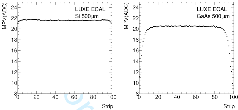
Fig. 18 Distribution of the MPV of the signal of a Si sensor (left) and a GaAs sensor (right) as a function of the strip number along the y coordinate.
