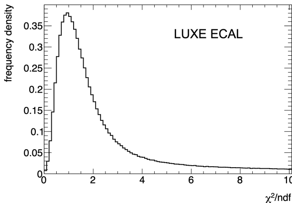
Fig. 12 The distribution of \chi^2/ndf ( \chi^2 per number of degrees of freedom) for electron trajectories fitted in the telescope.
