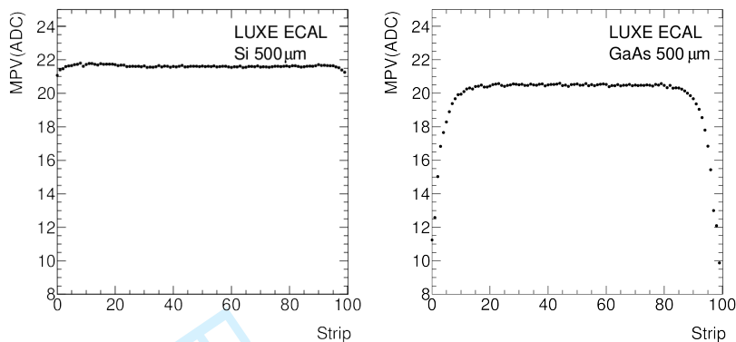
Fig. 19 Distribution of the MPV of the signal of a Si sensor (left) and a GaAs sensor (right) as a function of the strip number along the y coordinate.
