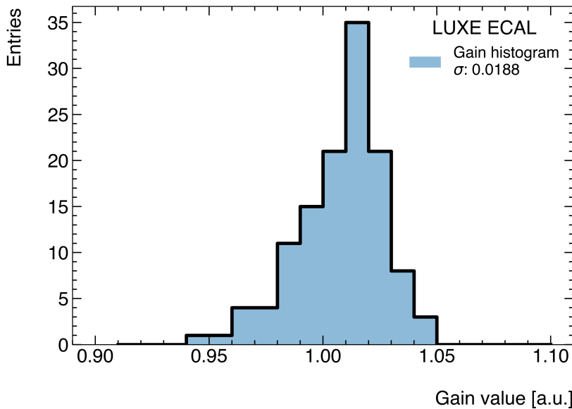
Fig. 9 The distribution of the normalised gains.
