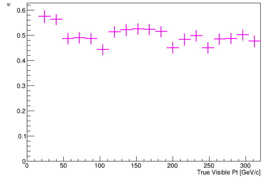
Pion Fake Rate by Electrons vs Pt
