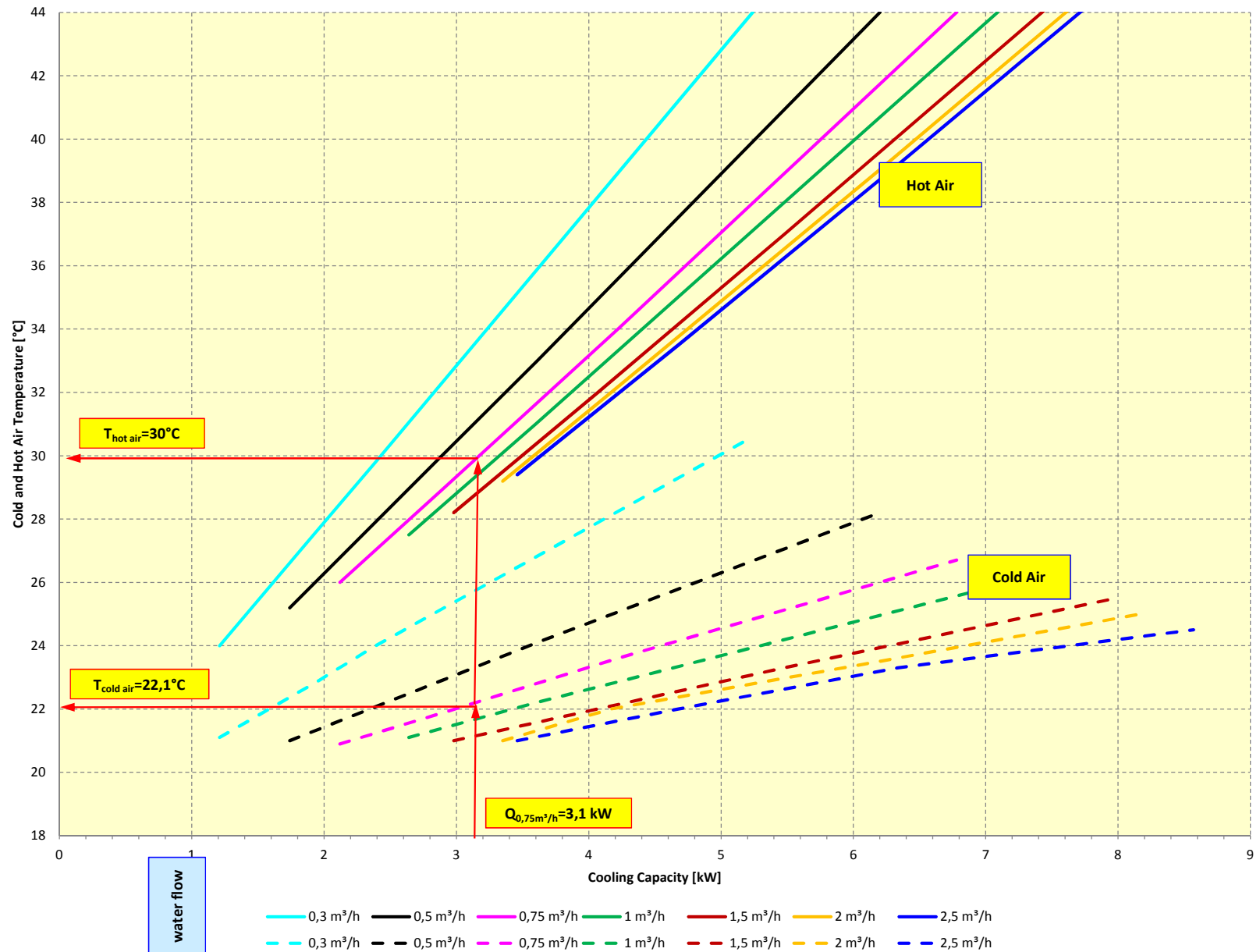
Cooling Diagram for T_{H_2O}=18^{\circ}\text{C}
